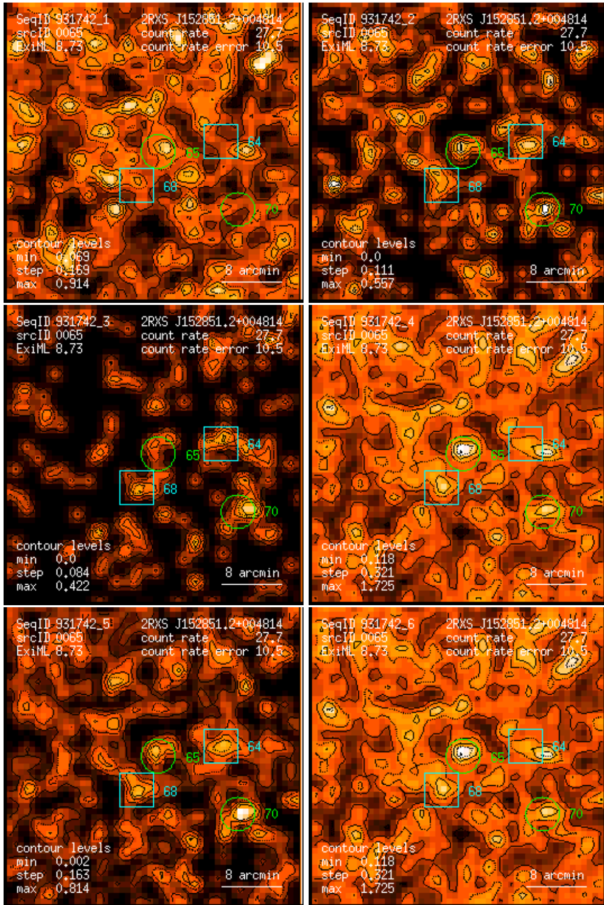
Figure 65: RASS 931742: detection 0065: band rate images, Gaussian filter: (1) PSPC channels 11 – 41, (2) 52 – 90, (3) 91 – 201, (4) 11 – 235, (5) 52 – 201, (6) 11 – 201. Broad band rates in counts/ks. Band rate contour levels in counts/ks/arcmin 2 .
