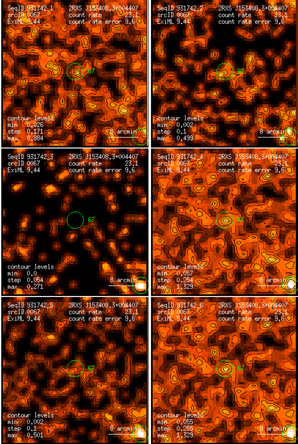
Figure 67: RASS 931742: detection 0067: band rate images, Gaussian filter: (1) PSPC channels 11 – 41, (2) 52 – 90, (3) 91 – 201, (4) 11 – 235, (5) 52 – 201, (6) 11 – 201. Broad band rates in counts/ks. Band rate contour levels in counts/ks/arcmin 2 .
