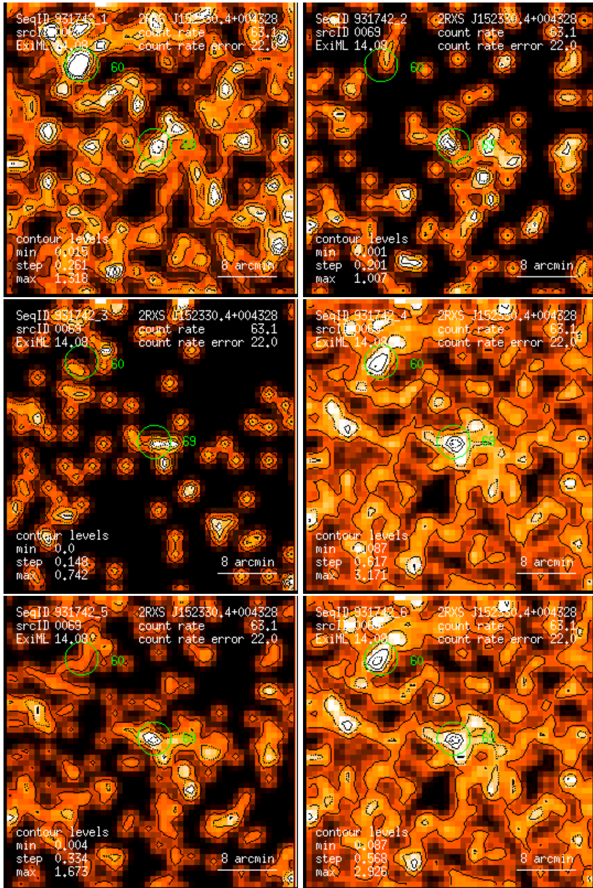
Figure 69: RASS 931742: detection 0069: band rate images, Gaussian filter: (1) PSPC channels 11 – 41, (2) 52 – 90, (3) 91 – 201, (4) 11 – 235, (5) 52 – 201, (6) 11 – 201. Broad band rates in counts/ks. Band rate contour levels in counts/ks/arcmin 2 .
