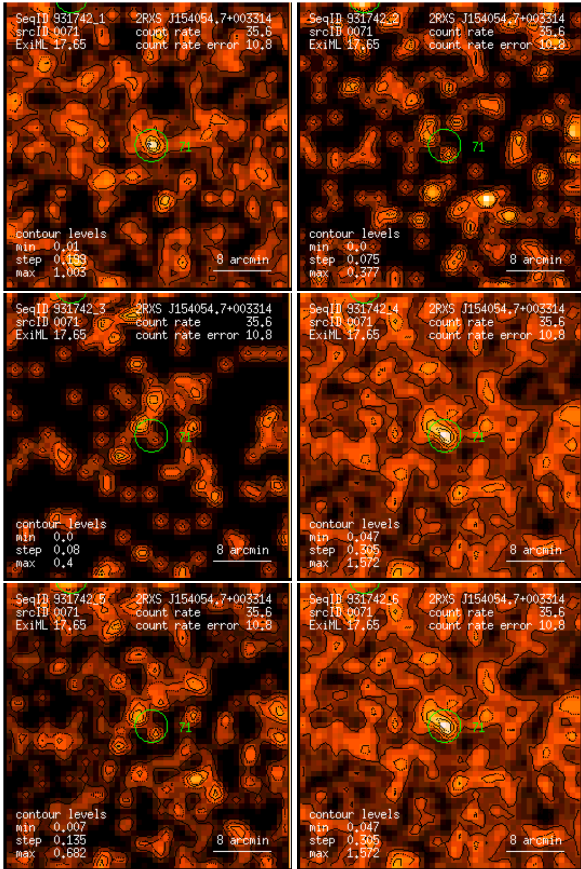
Figure 71: RASS 931742: detection 0071: band rate images, Gaussian filter: (1) PSPC channels 11 – 41, (2) 52 – 90, (3) 91 – 201, (4) 11 – 235, (5) 52 – 201, (6) 11 – 201. Broad band rates in counts/ks. Band rate contour levels in counts/ks/arcmin 2 .
