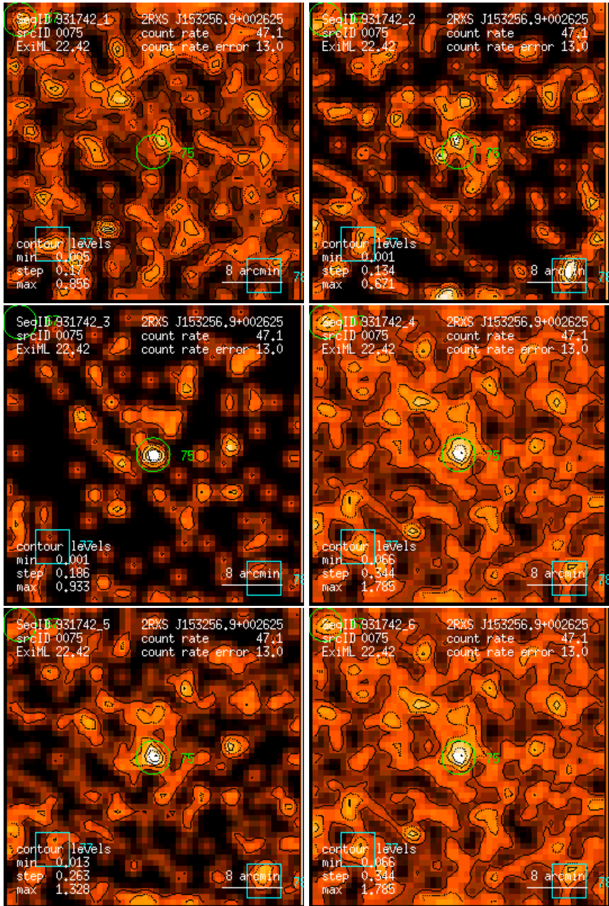
Figure 75: RASS 931742: detection 0075: band rate images, Gaussian filter: (1) PSPC channels 11 – 41, (2) 52 – 90, (3) 91 – 201, (4) 11 – 235, (5) 52 – 201, (6) 11 – 201. Broad band rates in counts/ks. Band rate contour levels in counts/ks/arcmin 2 .
