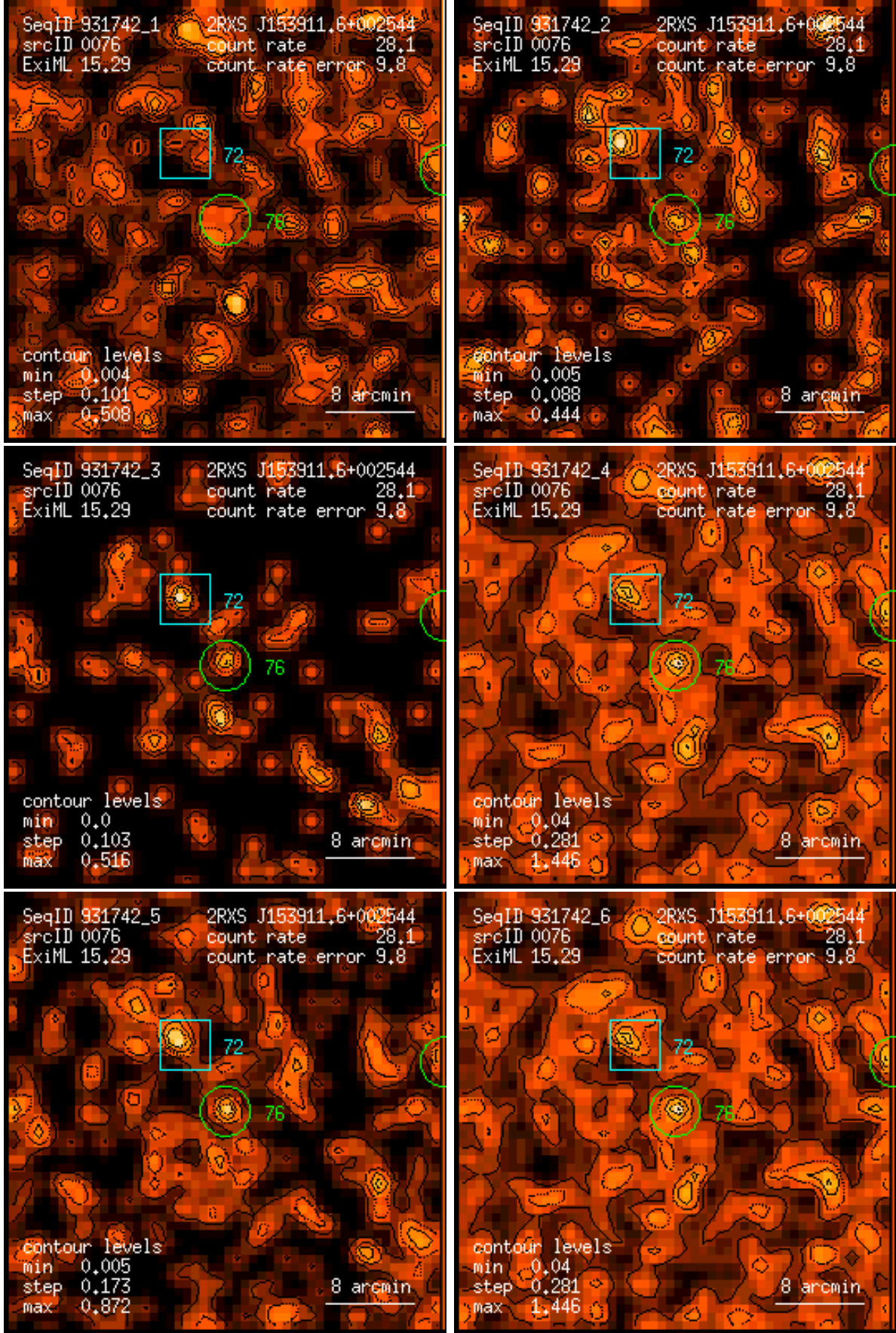
Figure 76: RASS 931742: detection 0076: band rate images, Gaussian filter: (1) PSPC channels 11 – 41, (2) 52 – 90, (3) 91 – 201, (4) 11 – 235, (5) 52 – 201, (6) 11 – 201. Broad band rates in counts/ks. Band rate contour levels in counts/ks/arcmin 2 .
