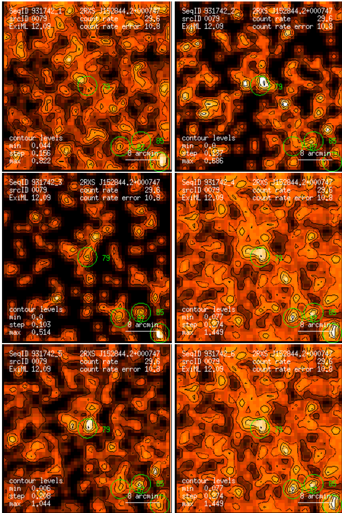
Figure 79: RASS 931742: detection 0079: band rate images, Gaussian filter: (1) PSPC channels 11 – 41, (2) 52 – 90, (3) 91 – 201, (4) 11 – 235, (5) 52 – 201, (6) 11 – 201. Broad band rates in counts/ks. Band rate contour levels in counts/ks/arcmin 2 .
