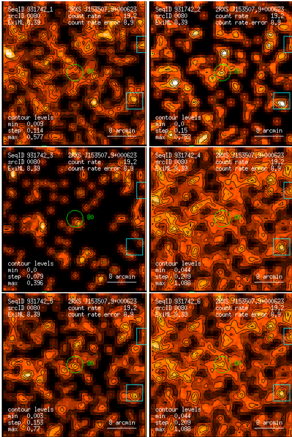
Figure 80: RASS 931742: detection 0080: band rate images, Gaussian filter: (1) PSPC channels 11 – 41, (2) 52 – 90, (3) 91 – 201, (4) 11 – 235, (5) 52 – 201, (6) 11 – 201. Broad band rates in counts/ks. Band rate contour levels in counts/ks/arcmin 2 .
