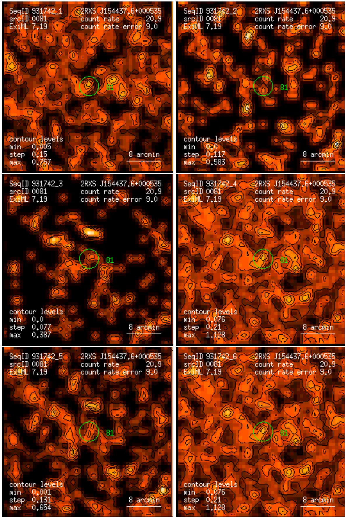
Figure 81: RASS 931742: detection 0081: band rate images, Gaussian filter: (1) PSPC channels 11 – 41, (2) 52 – 90, (3) 91 – 201, (4) 11 – 235, (5) 52 – 201, (6) 11 – 201. Broad band rates in counts/ks. Band rate contour levels in counts/ks/arcmin 2 .
