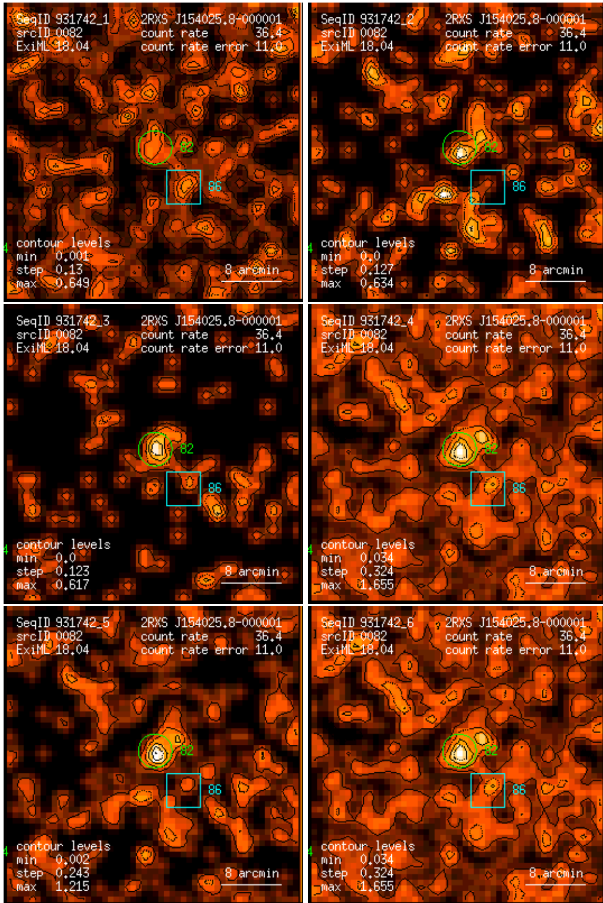
Figure 82: RASS 931742: detection 0082: band rate images, Gaussian filter: (1) PSPC channels 11 – 41, (2) 52 – 90, (3) 91 – 201, (4) 11 – 235, (5) 52 – 201, (6) 11 – 201. Broad band rates in counts/ks. Band rate contour levels in counts/ks/arcmin 2 .
