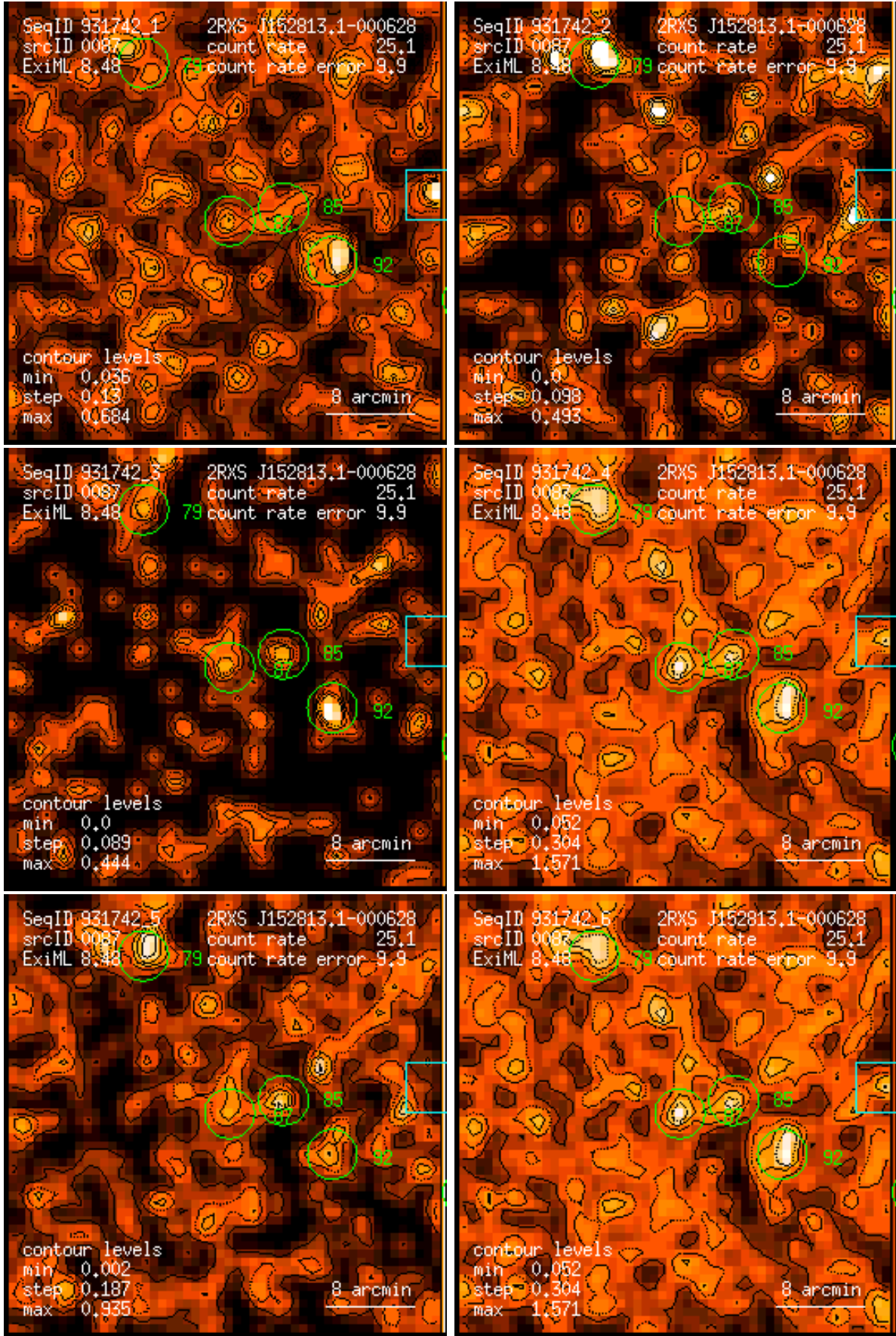
Figure 87: RASS 931742: detection 0087: band rate images, Gaussian filter: (1) PSPC channels 11 – 41, (2) 52 – 90, (3) 91 – 201, (4) 11 – 235, (5) 52 – 201, (6) 11 – 201. Broad band rates in counts/ks. Band rate contour levels in counts/ks/arcmin 2 .
