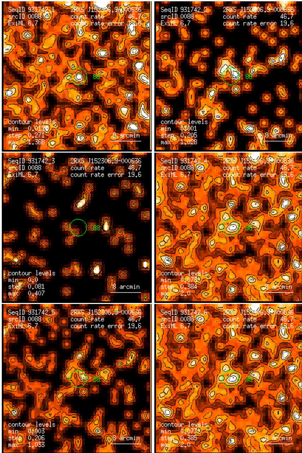
Figure 88: RASS 931742: detection 0088: band rate images, Gaussian filter: (1) PSPC channels 11 – 41, (2) 52 – 90, (3) 91 – 201, (4) 11 – 235, (5) 52 – 201, (6) 11 – 201. Broad band rates in counts/ks. Band rate contour levels in counts/ks/arcmin 2 .
