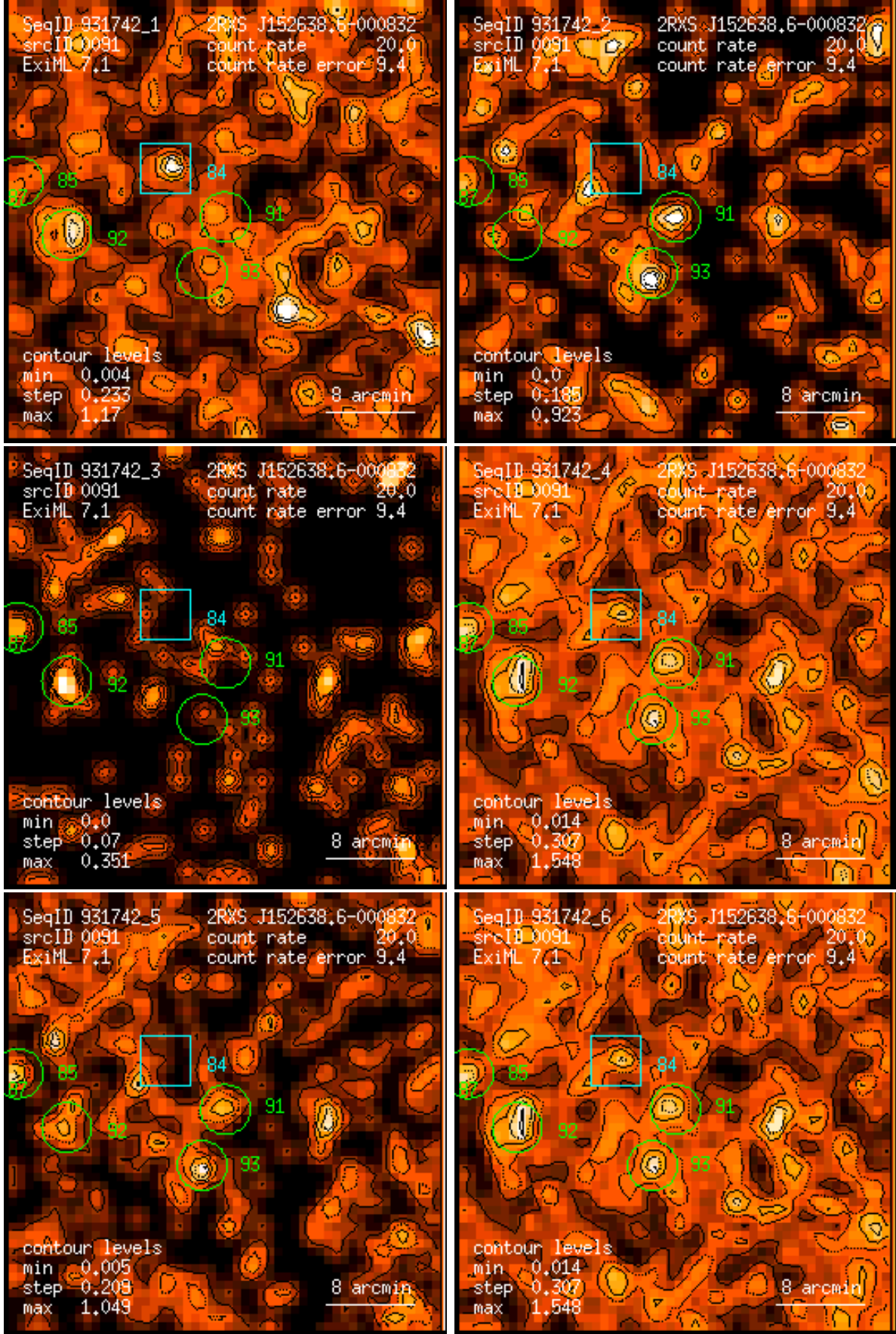
Figure 91: RASS 931742: detection 0091: band rate images, Gaussian filter: (1) PSPC channels 11 – 41, (2) 52 – 90, (3) 91 – 201, (4) 11 – 235, (5) 52 – 201, (6) 11 – 201. Broad band rates in counts/ks. Band rate contour levels in counts/ks/arcmin 2 .
