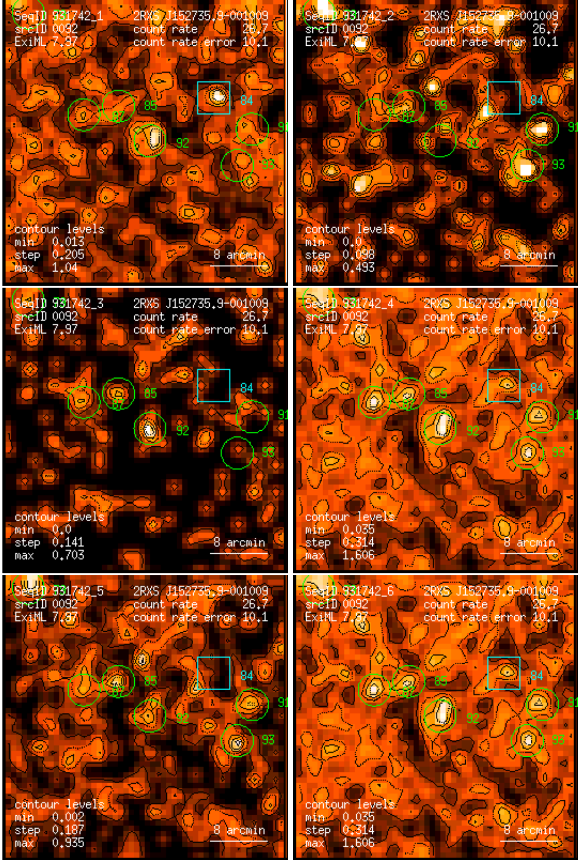
Figure 92: RASS 931742: detection 0092: band rate images, Gaussian filter: (1) PSPC channels 11 – 41, (2) 52 – 90, (3) 91 – 201, (4) 11 – 235, (5) 52 – 201, (6) 11 – 201. Broad band rates in counts/ks. Band rate contour levels in counts/ks/arcmin 2 .
