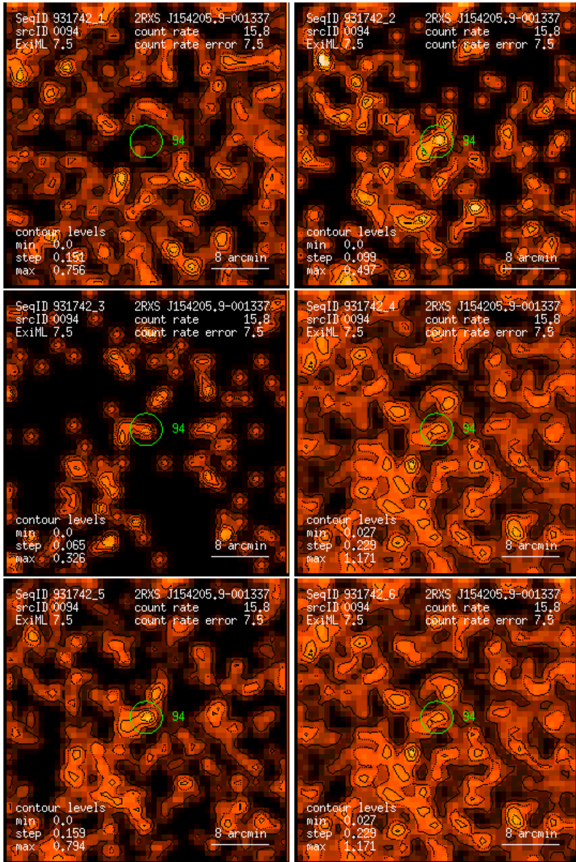
Figure 94: RASS 931742: detection 0094: band rate images, Gaussian filter: (1) PSPC channels 11 – 41, (2) 52 – 90, (3) 91 – 201, (4) 11 – 235, (5) 52 – 201, (6) 11 – 201. Broad band rates in counts/ks. Band rate contour levels in counts/ks/arcmin 2 .
