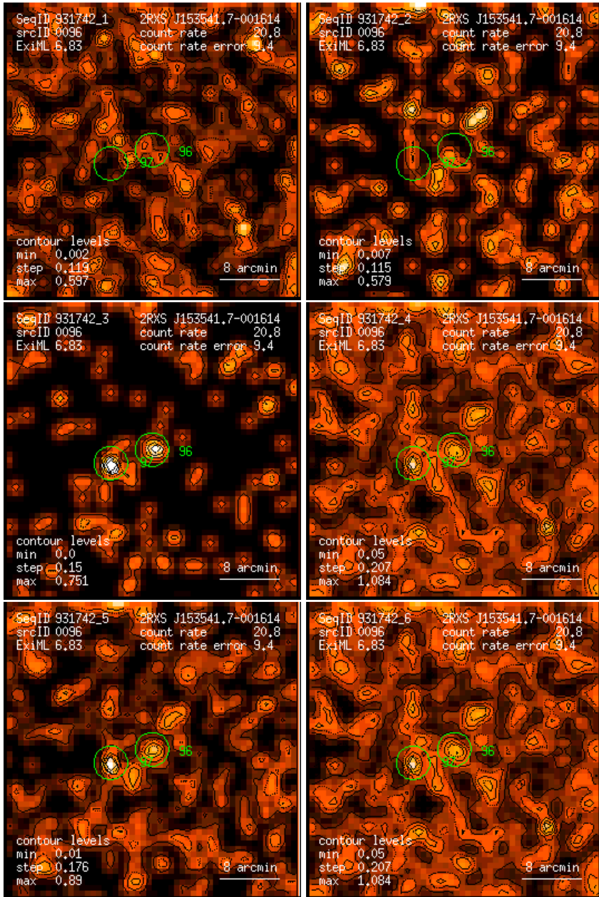
Figure 96: RASS 931742: detection 0096: band rate images, Gaussian filter: (1) PSPC channels 11 – 41, (2) 52 – 90, (3) 91 – 201, (4) 11 – 235, (5) 52 – 201, (6) 11 – 201. Broad band rates in counts/ks. Band rate contour levels in counts/ks/arcmin 2 .
