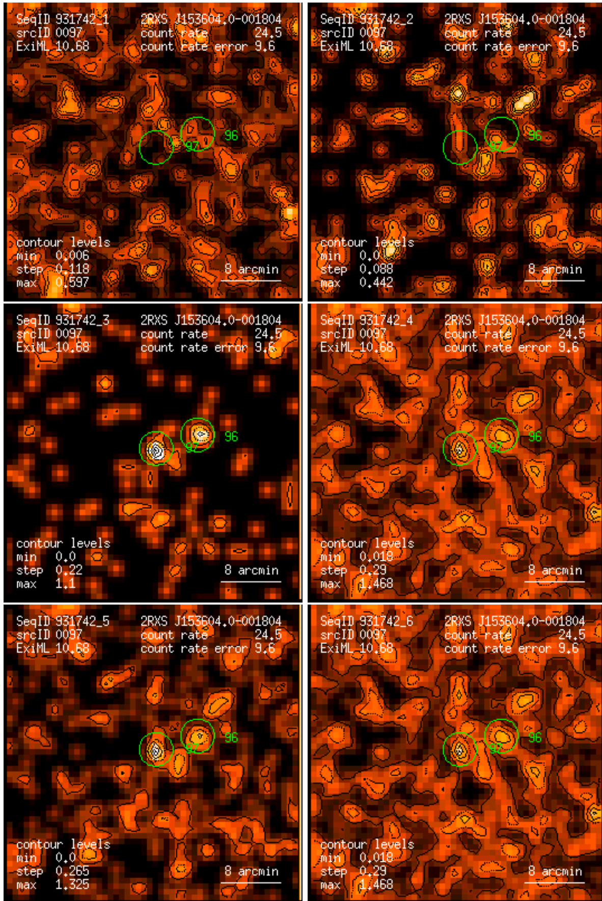
Figure 97: RASS 931742: detection 0097: band rate images, Gaussian filter: (1) PSPC channels 11 – 41, (2) 52 – 90, (3) 91 – 201, (4) 11 – 235, (5) 52 – 201, (6) 11 – 201. Broad band rates in counts/ks. Band rate contour levels in counts/ks/arcmin 2 .
