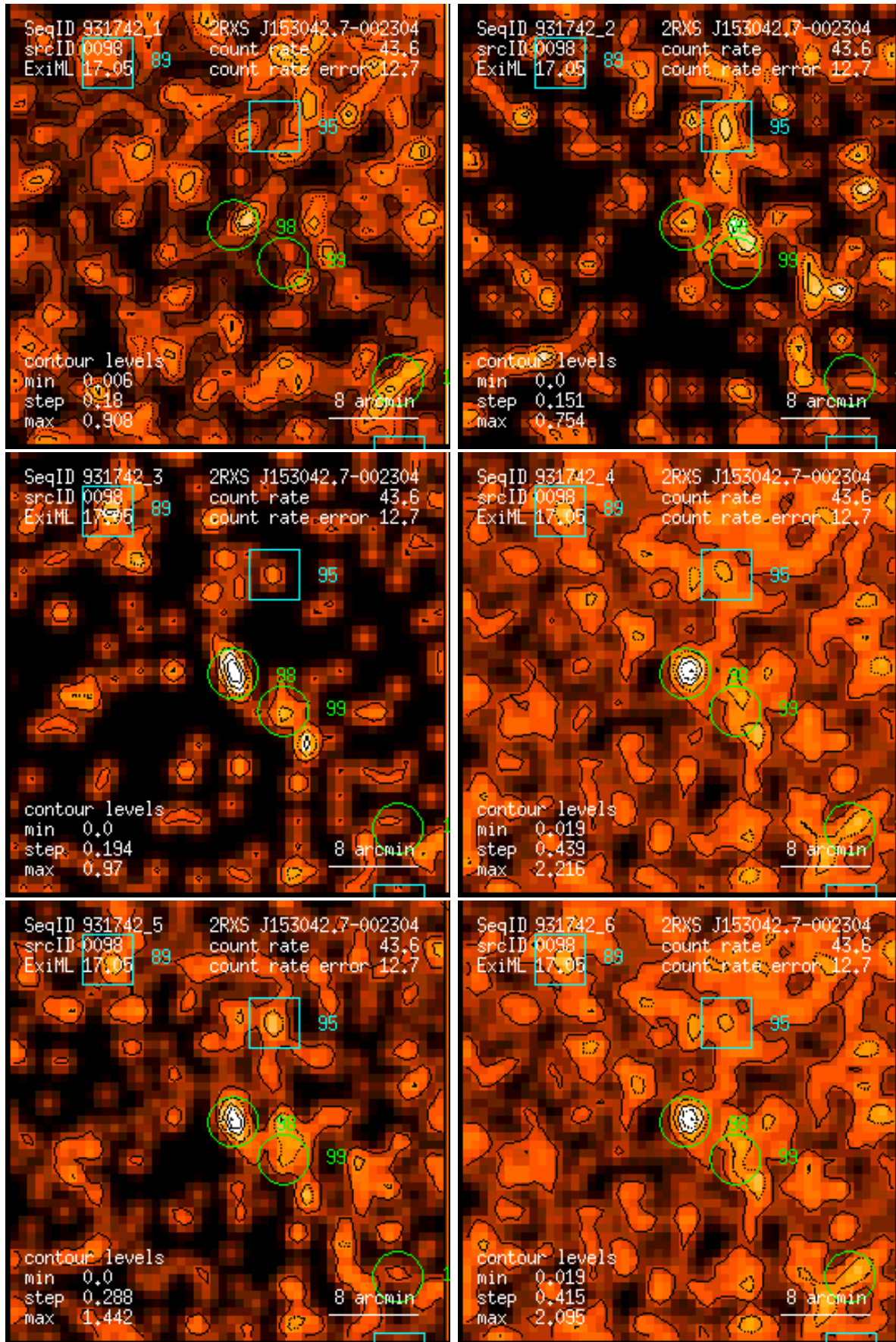
Figure 98: RASS 931742: detection 0098: band rate images, Gaussian filter: (1) PSPC channels 11 – 41, (2) 52 – 90, (3) 91 – 201, (4) 11 – 235, (5) 52 – 201, (6) 11 – 201. Broad band rates in counts/ks. Band rate contour levels in counts/ks/arcmin 2 .
