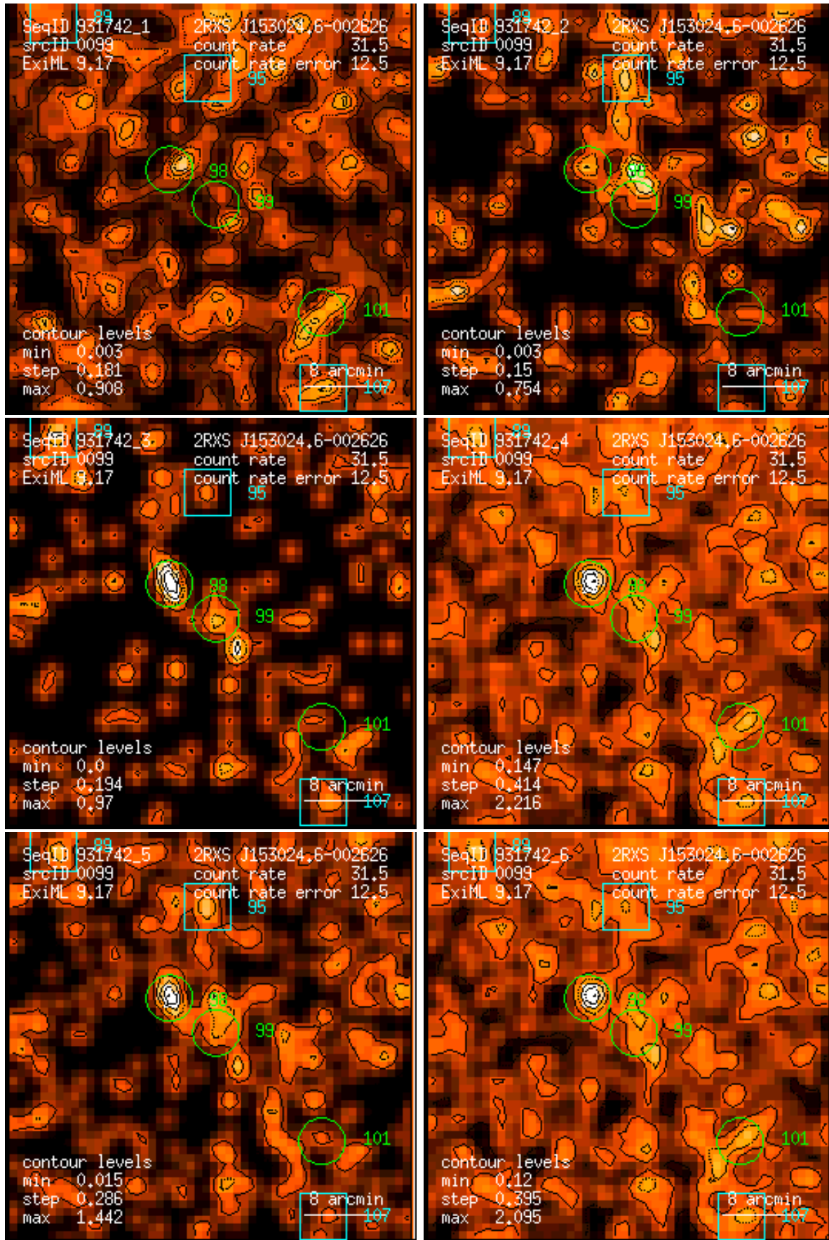
Figure 99: RASS 931742: detection 0099: band rate images, Gaussian filter: (1) PSPC channels 11 – 41, (2) 52 – 90, (3) 91 – 201, (4) 11 – 235, (5) 52 – 201, (6) 11 – 201. Broad band rates in counts/ks. Band rate contour levels in counts/ks/arcmin 2 .
