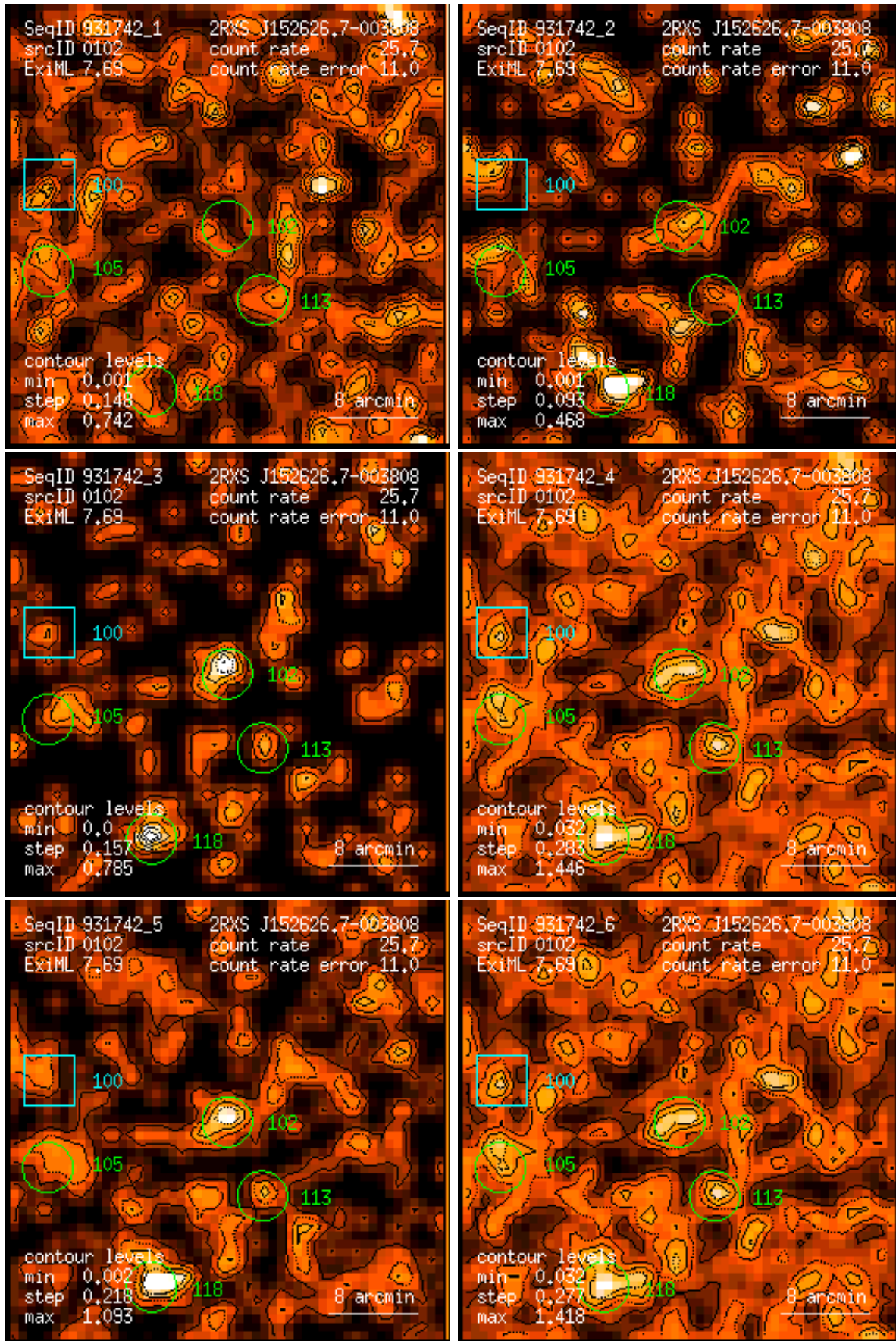
Figure 102: RASS 931742: detection 0102: band rate images, Gaussian filter: (1) PSPC channels 11 – 41, (2) 52 – 90, (3) 91 – 201, (4) 11 – 235, (5) 52 – 201, (6) 11 – 201. Broad band rates in counts/ks. Band rate contour levels in counts/ks/arcmin 2 .
