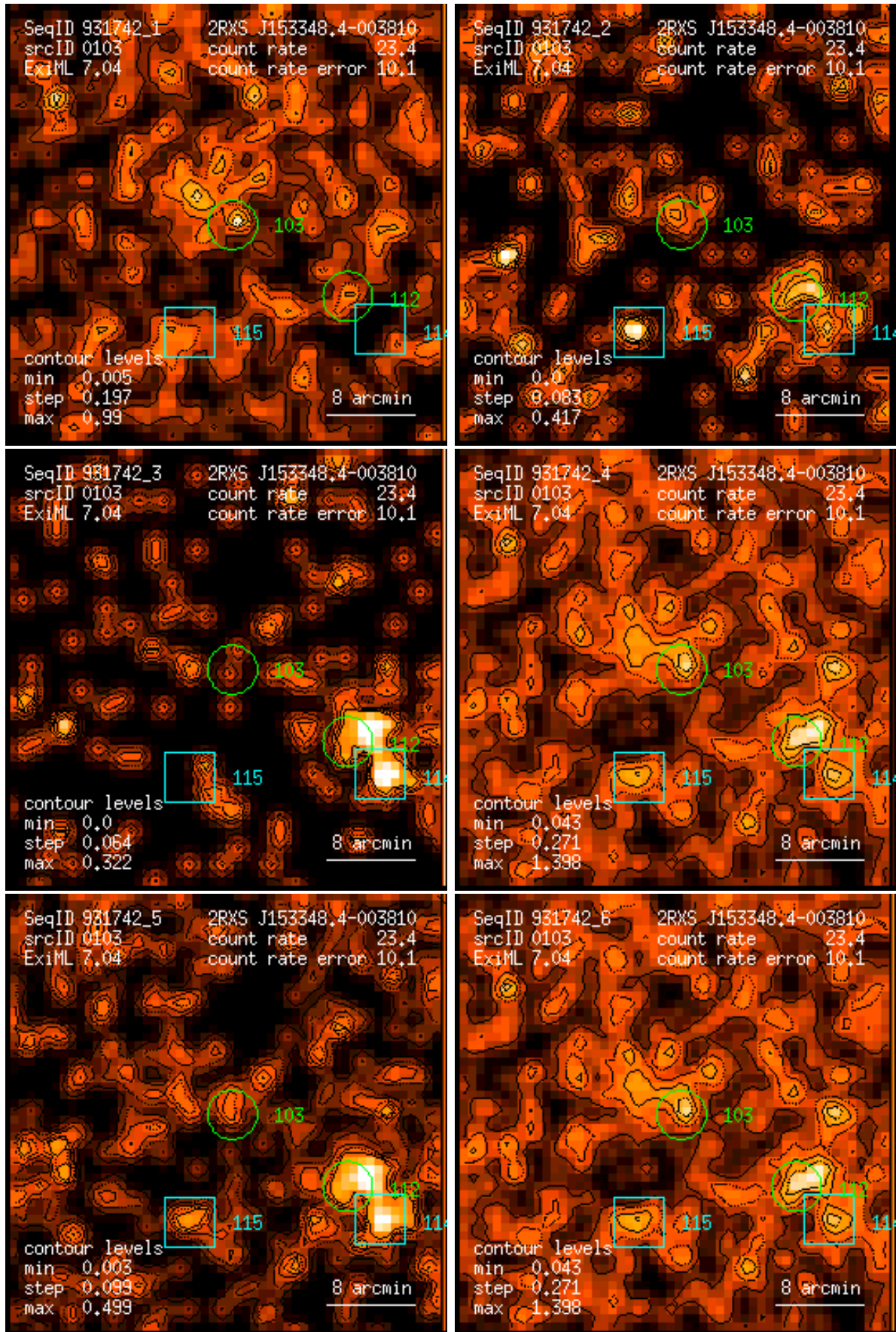
Figure 103: RASS 931742: detection 0103: band rate images, Gaussian filter: (1) PSPC channels 11 – 41, (2) 52 – 90, (3) 91 – 201, (4) 11 – 235, (5) 52 – 201, (6) 11 – 201. Broad band rates in counts/ks. Band rate contour levels in counts/ks/arcmin 2 .
