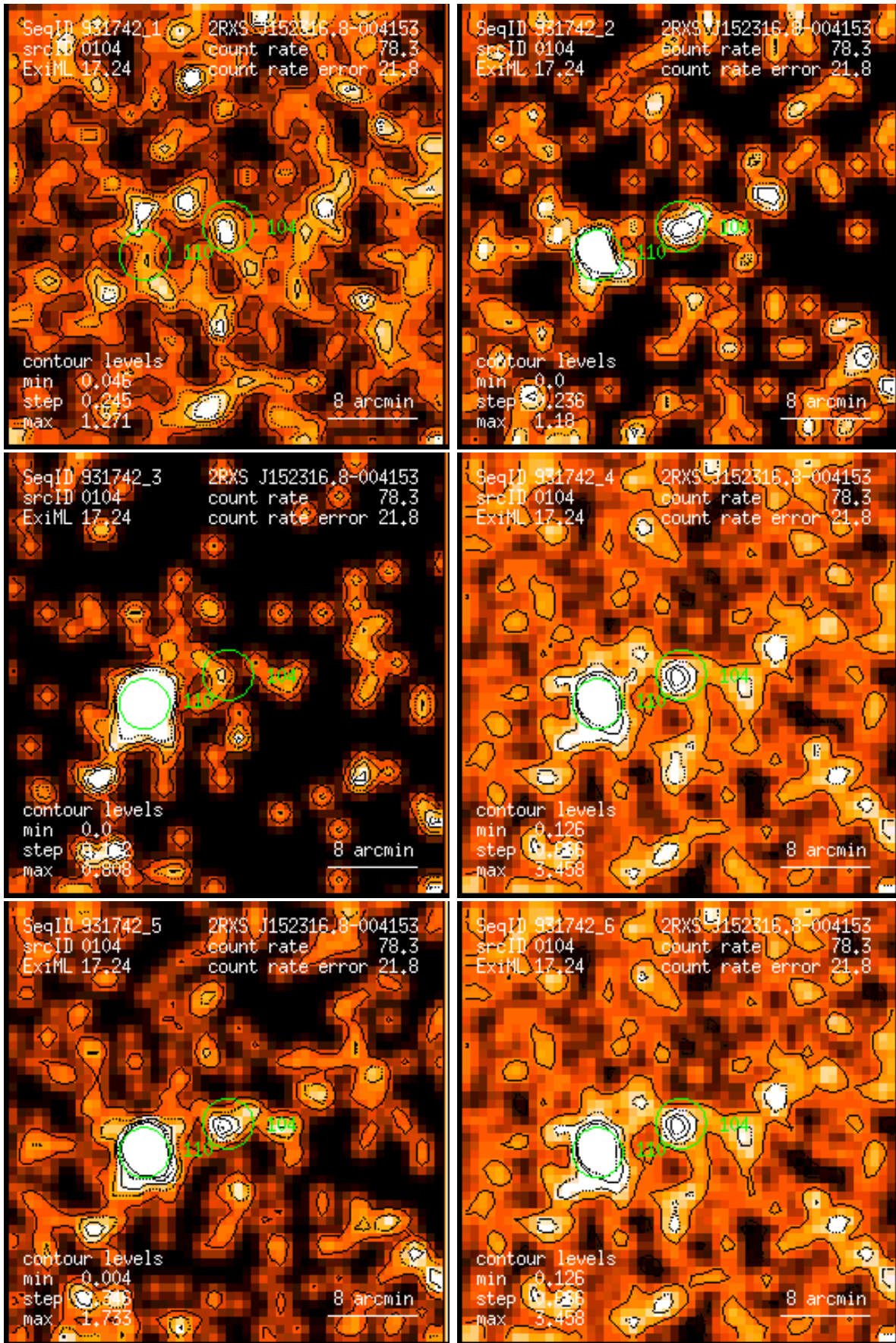
Figure 104: RASS 931742: detection 0104: band rate images, Gaussian filter: (1) PSPC channels 11 – 41, (2) 52 – 90, (3) 91 – 201, (4) 11 – 235, (5) 52 – 201, (6) 11 – 201. Broad band rates in counts/ks. Band rate contour levels in counts/ks/arcmin 2 .
