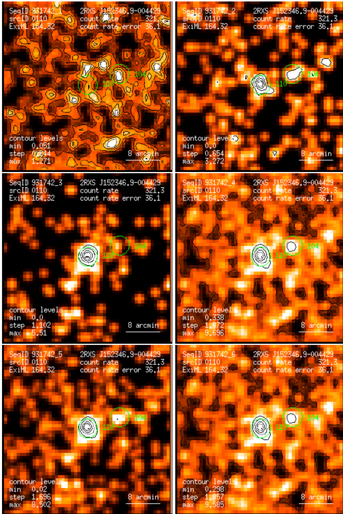
Figure 110: RASS 931742: detection 0110: band rate images, Gaussian filter: (1) PSPC channels 11 – 41, (2) 52 – 90, (3) 91 – 201, (4) 11 – 235, (5) 52 – 201, (6) 11 – 201. Broad band rates in counts/ks. Band rate contour levels in counts/ks/arcmin 2 .
