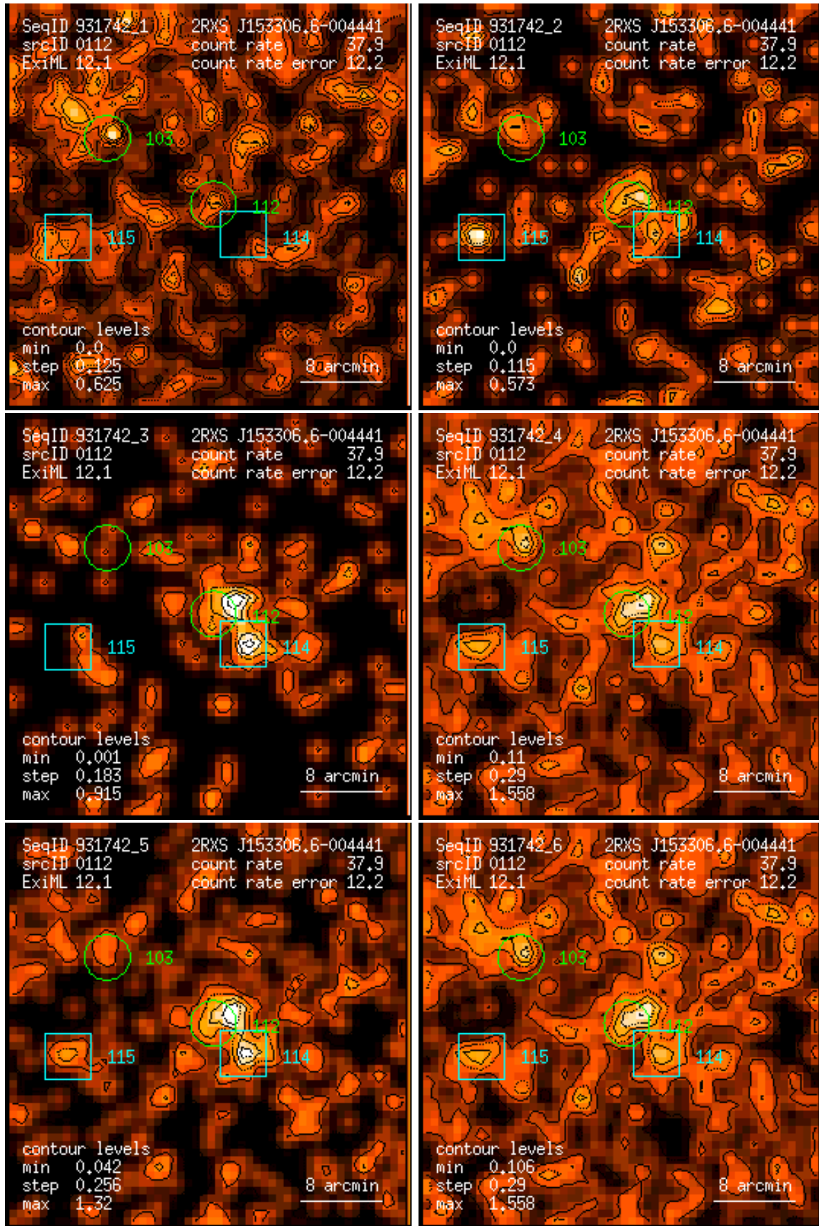
Figure 112: RASS 931742: detection 0112: band rate images, Gaussian filter: (1) PSPC channels 11 – 41, (2) 52 – 90, (3) 91 – 201, (4) 11 – 235, (5) 52 – 201, (6) 11 – 201. Broad band rates in counts/ks. Band rate contour levels in counts/ks/arcmin 2 .
