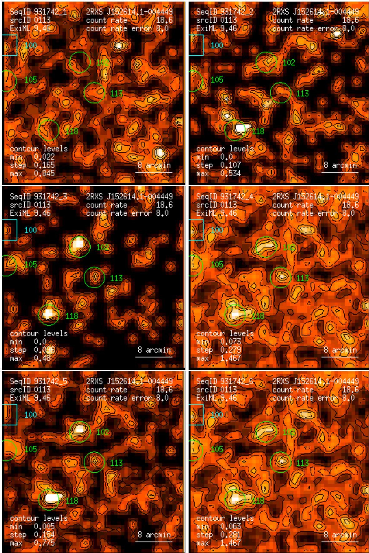
Figure 113: RASS 931742: detection 0113: band rate images, Gaussian filter: (1) PSPC channels 11 – 41, (2) 52 – 90, (3) 91 – 201, (4) 11 – 235, (5) 52 – 201, (6) 11 – 201. Broad band rates in counts/ks. Band rate contour levels in counts/ks/arcmin 2 .
