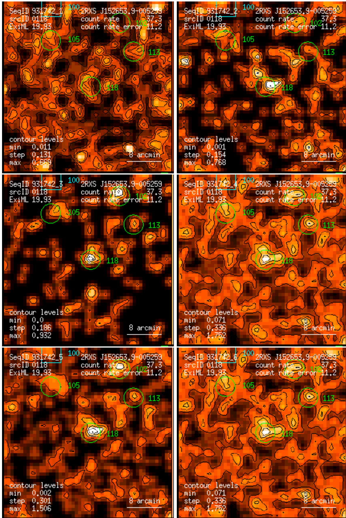
Figure 118: RASS 931742: detection 0118: band rate images, Gaussian filter: (1) PSPC channels 11 – 41, (2) 52 – 90, (3) 91 – 201, (4) 11 – 235, (5) 52 – 201, (6) 11 – 201. Broad band rates in counts/ks. Band rate contour levels in counts/ks/arcmin 2 .
