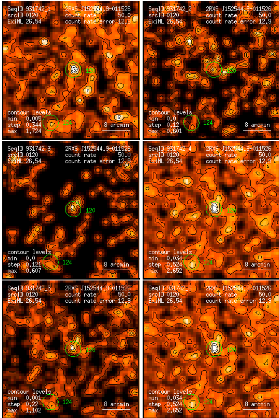
Figure 120: RASS 931742: detection 0120: band rate images, Gaussian filter: (1) PSPC channels 11 – 41, (2) 52 – 90, (3) 91 – 201, (4) 11 – 235, (5) 52 – 201, (6) 11 – 201. Broad band rates in counts/ks. Band rate contour levels in counts/ks/arcmin 2 .
