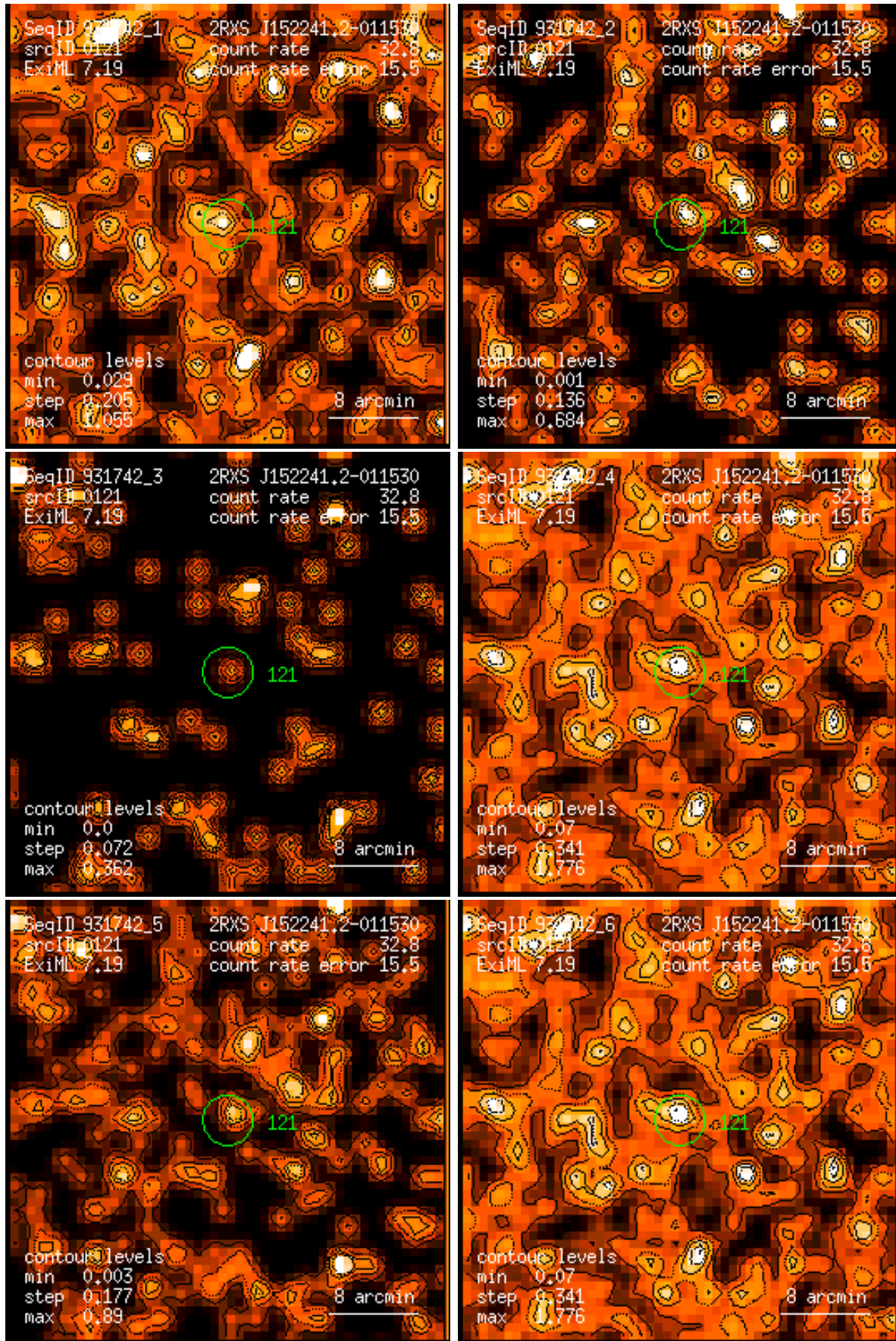
Figure 121: RASS 931742: detection 0121: band rate images, Gaussian filter: (1) PSPC channels 11 – 41, (2) 52 – 90, (3) 91 – 201, (4) 11 – 235, (5) 52 – 201, (6) 11 – 201. Broad band rates in counts/ks. Band rate contour levels in counts/ks/arcmin 2 .
