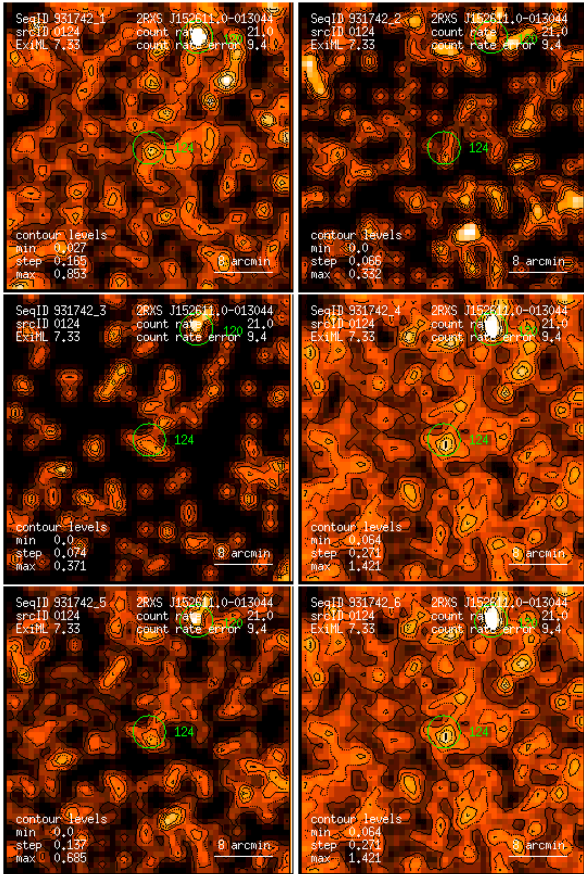
Figure 124: RASS 931742: detection 0124: band rate images, Gaussian filter: (1) PSPC channels 11 – 41, (2) 52 – 90, (3) 91 – 201, (4) 11 – 235, (5) 52 – 201, (6) 11 – 201. Broad band rates in counts/ks. Band rate contour levels in counts/ks/arcmin 2 .
