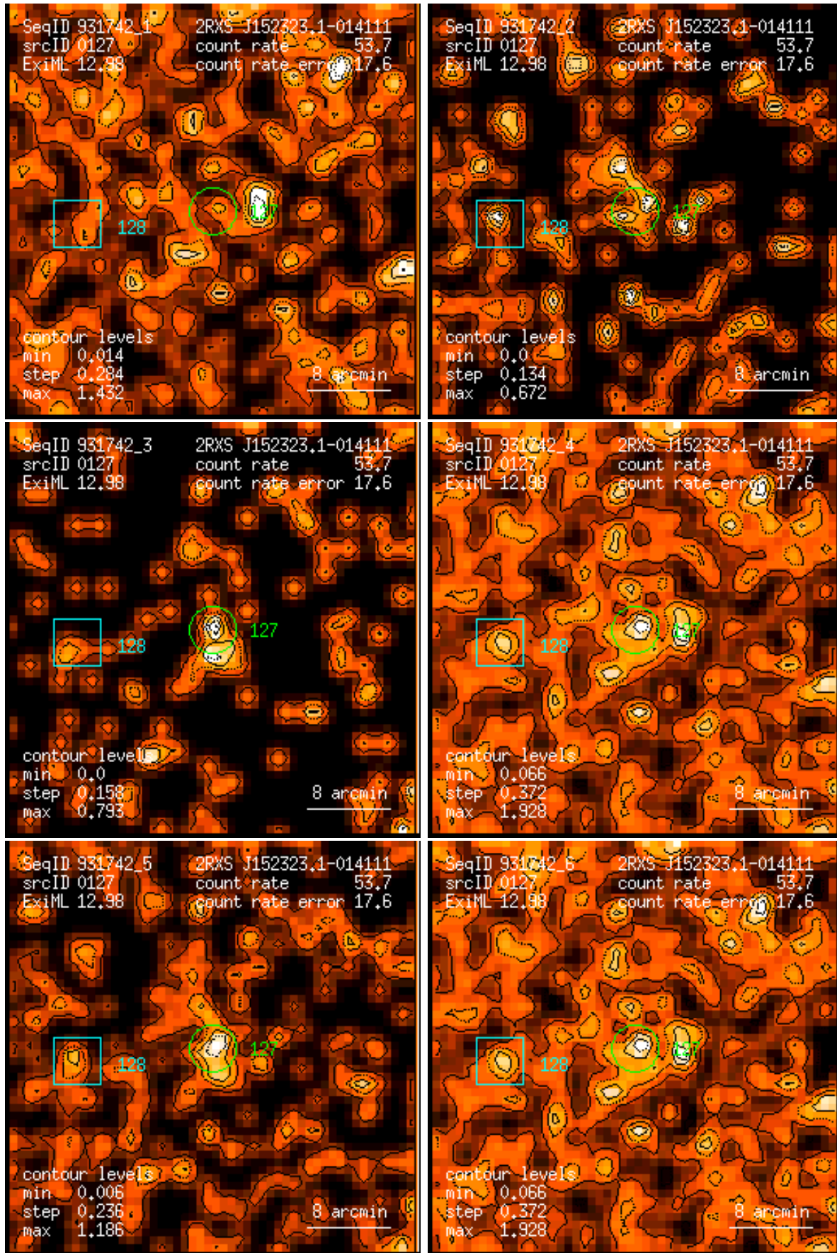
Figure 127: RASS 931742: detection 0127: band rate images, Gaussian filter: (1) PSPC channels 11 – 41, (2) 52 – 90, (3) 91 – 201, (4) 11 – 235, (5) 52 – 201, (6) 11 – 201. Broad band rates in counts/ks. Band rate contour levels in counts/ks/arcmin 2 .
