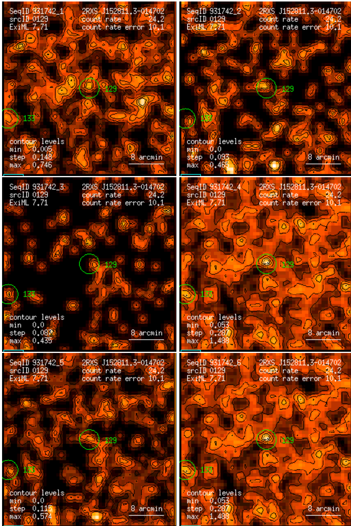
Figure 129: RASS 931742: detection 0129: band rate images, Gaussian filter: (1) PSPC channels 11 – 41, (2) 52 – 90, (3) 91 – 201, (4) 11 – 235, (5) 52 – 201, (6) 11 – 201. Broad band rates in counts/ks. Band rate contour levels in counts/ks/arcmin 2 .
