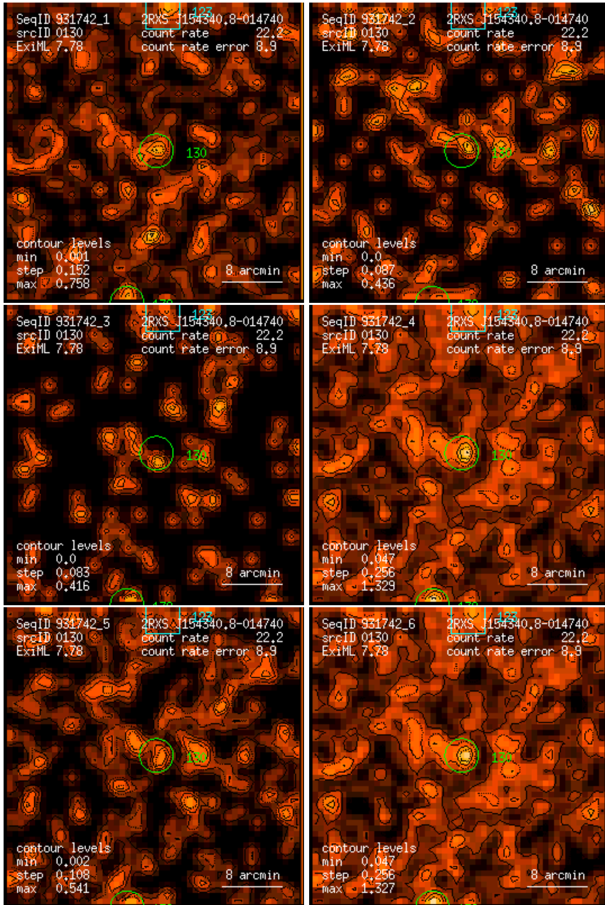
Figure 130: RASS 931742: detection 0130: band rate images, Gaussian filter: (1) PSPC channels 11 – 41, (2) 52 – 90, (3) 91 – 201, (4) 11 – 235, (5) 52 – 201, (6) 11 – 201. Broad band rates in counts/ks. Band rate contour levels in counts/ks/arcmin 2 .
