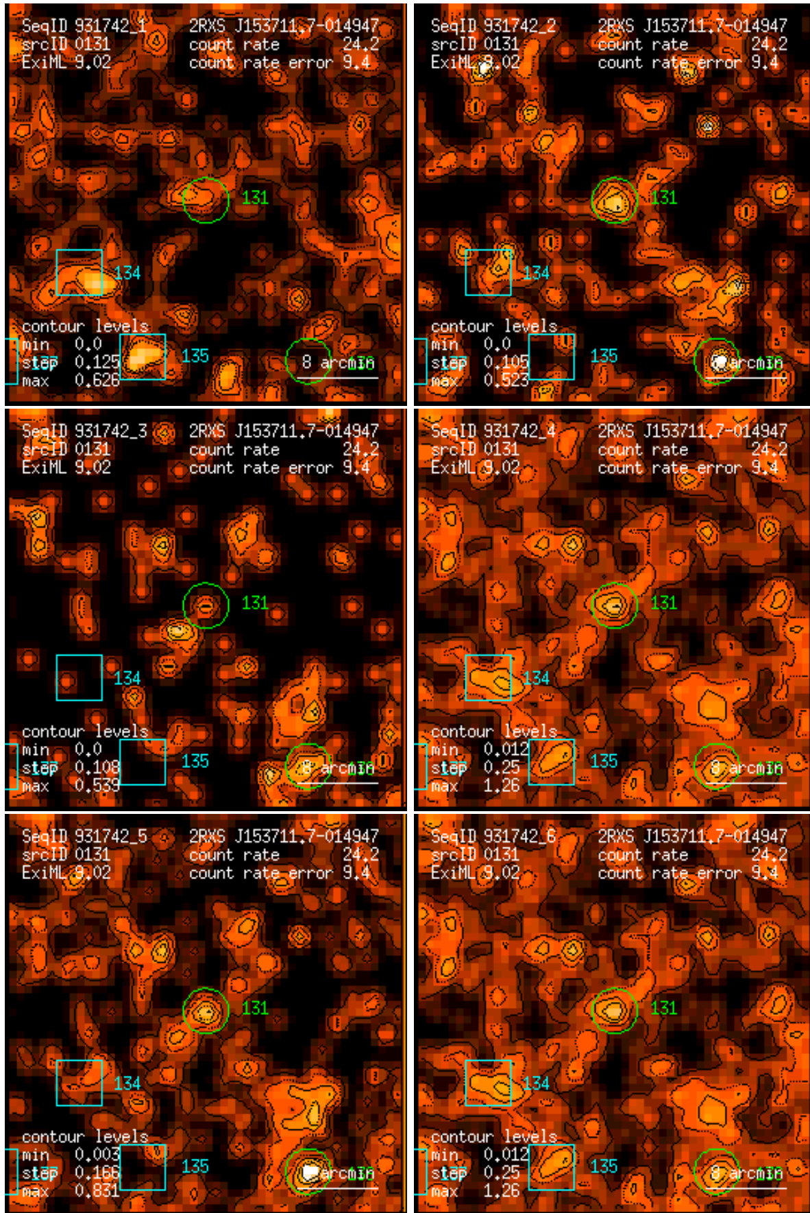
Figure 131: RASS 931742: detection 0131: band rate images, Gaussian filter: (1) PSPC channels 11 – 41, (2) 52 – 90, (3) 91 – 201, (4) 11 – 235, (5) 52 – 201, (6) 11 – 201. Broad band rates in counts/ks. Band rate contour levels in counts/ks/arcmin 2 .
