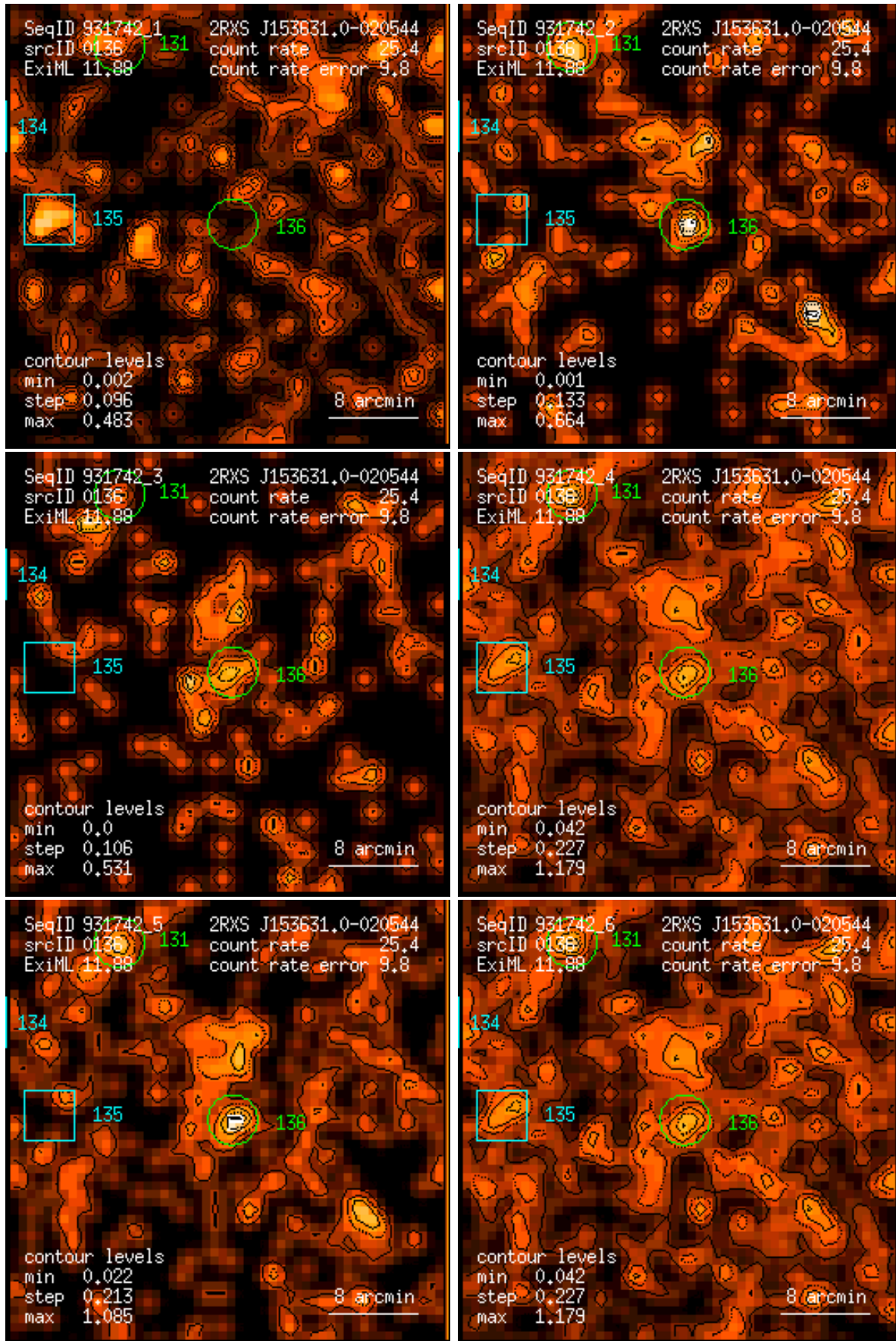
Figure 136: RASS 931742: detection 0136: band rate images, Gaussian filter: (1) PSPC channels 11 – 41, (2) 52 – 90, (3) 91 – 201, (4) 11 – 235, (5) 52 – 201, (6) 11 – 201. Broad band rates in counts/ks. Band rate contour levels in counts/ks/arcmin 2 .
