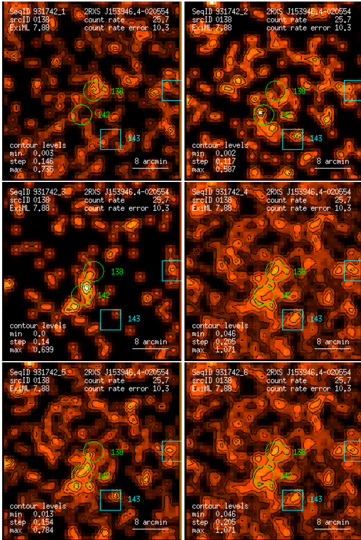
Figure 138: RASS 931742: detection 0138: band rate images, Gaussian filter: (1) PSPC channels 11 – 41, (2) 52 – 90, (3) 91 – 201, (4) 11 – 235, (5) 52 – 201, (6) 11 – 201. Broad band rates in counts/ks. Band rate contour levels in counts/ks/arcmin 2 .
