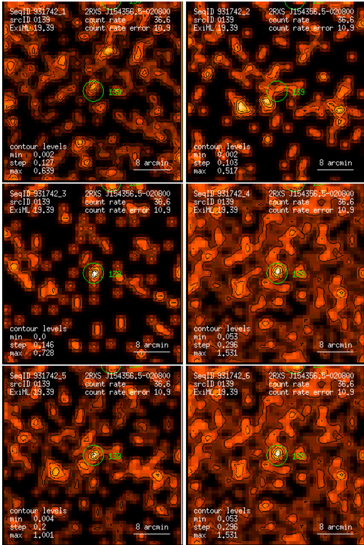
Figure 139: RASS 931742: detection 0139: band rate images, Gaussian filter: (1) PSPC channels 11 – 41, (2) 52 – 90, (3) 91 – 201, (4) 11 – 235, (5) 52 – 201, (6) 11 – 201. Broad band rates in counts/ks. Band rate contour levels in counts/ks/arcmin 2 .
