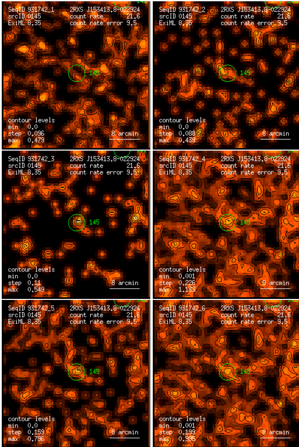
Figure 145: RASS 931742: detection 0145: band rate images, Gaussian filter: (1) PSPC channels 11 – 41, (2) 52 – 90, (3) 91 – 201, (4) 11 – 235, (5) 52 – 201, (6) 11 – 201. Broad band rates in counts/ks. Band rate contour levels in counts/ks/arcmin 2 .
