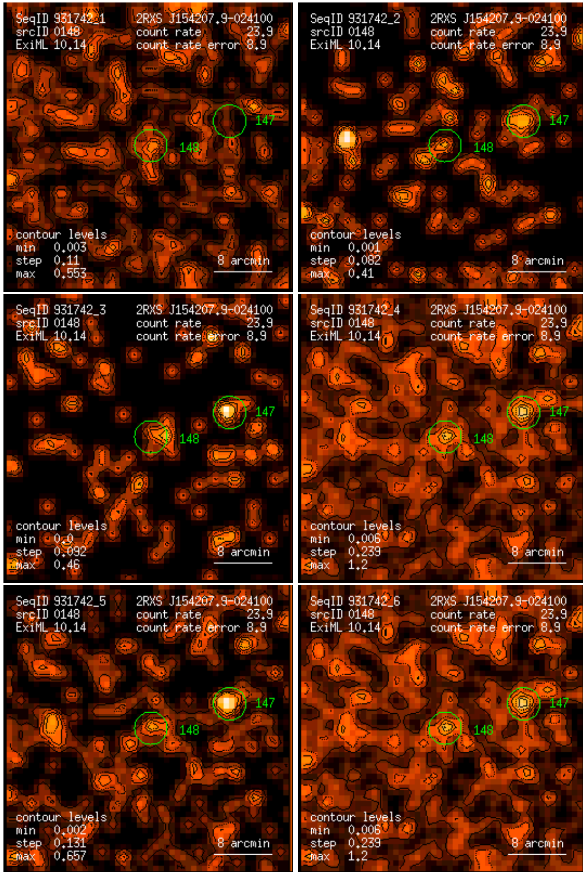
Figure 148: RASS 931742: detection 0148: band rate images, Gaussian filter: (1) PSPC channels 11 – 41, (2) 52 – 90, (3) 91 – 201, (4) 11 – 235, (5) 52 – 201, (6) 11 – 201. Broad band rates in counts/ks. Band rate contour levels in counts/ks/arcmin 2 .
