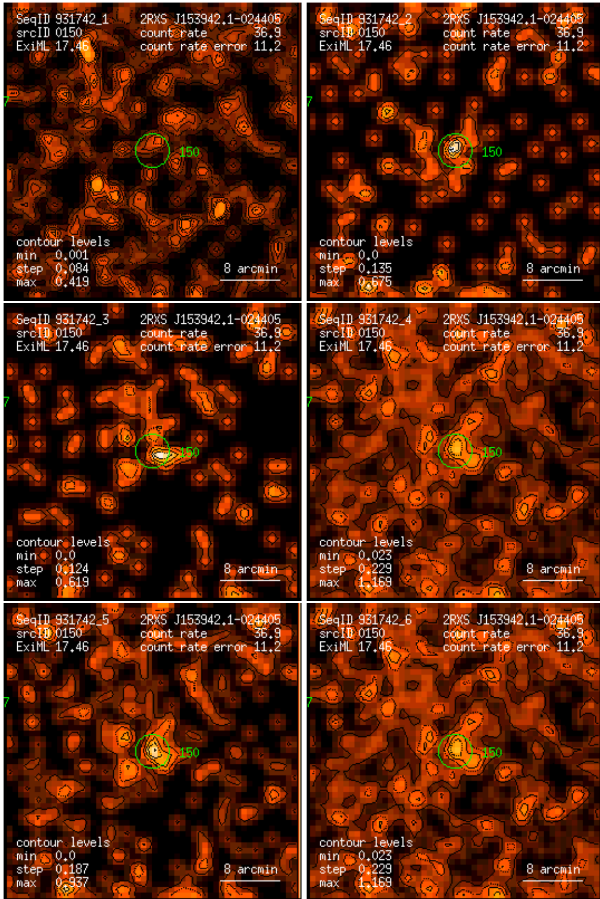
Figure 150: RASS 931742: detection 0150: band rate images, Gaussian filter: (1) PSPC channels 11 – 41, (2) 52 – 90, (3) 91 – 201, (4) 11 – 235, (5) 52 – 201, (6) 11 – 201. Broad band rates in counts/ks. Band rate contour levels in counts/ks/arcmin 2 .
