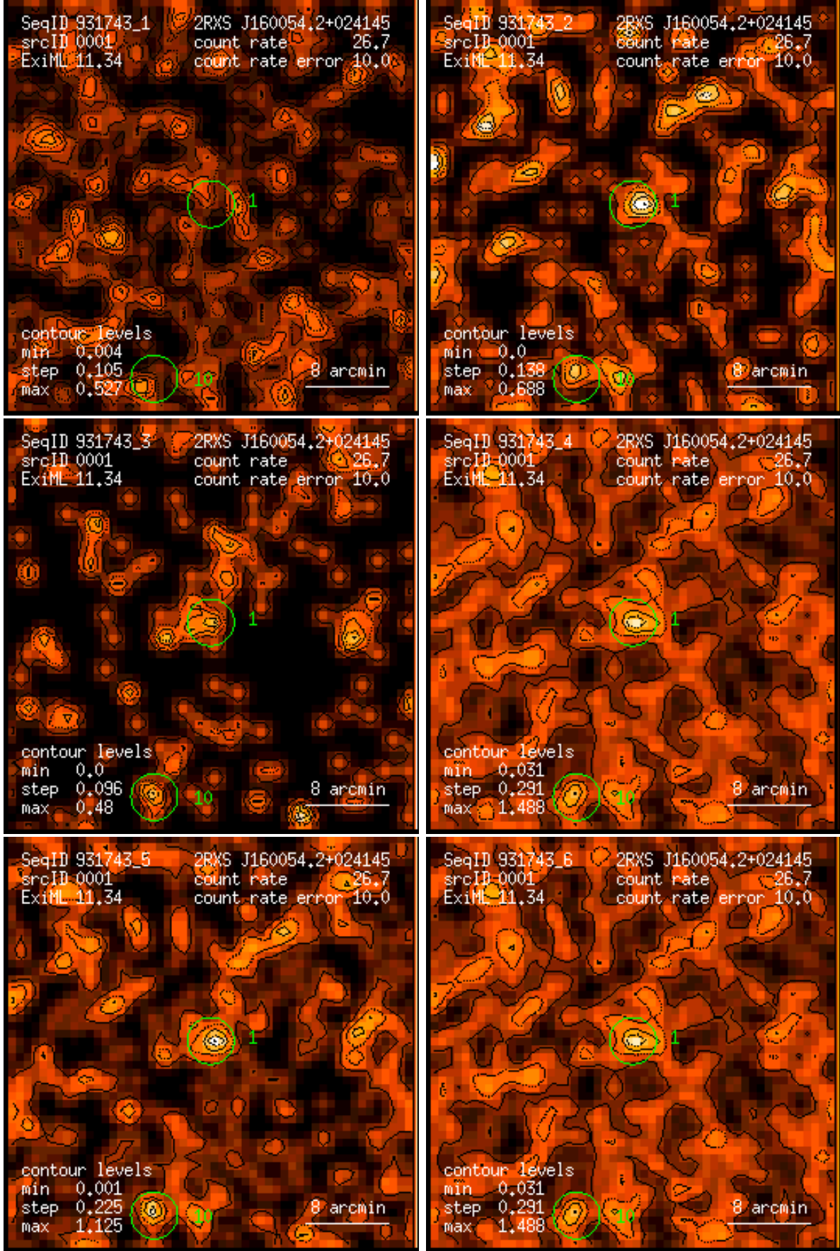
Figure 1: RASS 931743: detection 0001: band rate images, Gaussian filter: (1) PSPC channels 11 – 41, (2) 52 – 90, (3) 91 – 201, (4) 11 – 235, (5) 52 – 201, (6) 11 – 201. Broad band rates in counts/ks. Band rate contour levels in counts/ks/arcmin 2 .
