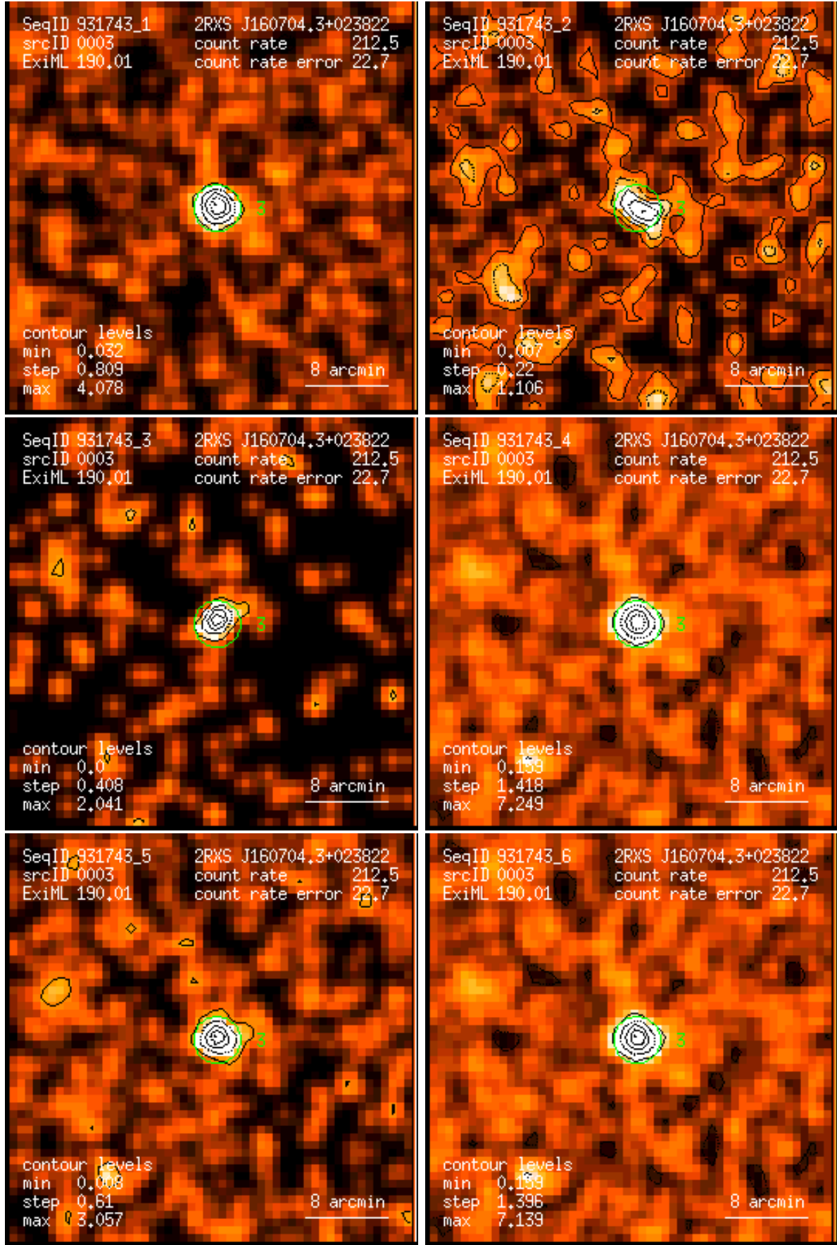
Figure 3: RASS 931743: detection 0003: band rate images, Gaussian filter: (1) PSPC channels 11 – 41, (2) 52 – 90, (3) 91 – 201, (4) 11 – 235, (5) 52 – 201, (6) 11 – 201. Broad band rates in counts/ks. Band rate contour levels in counts/ks/arcmin 2 .
