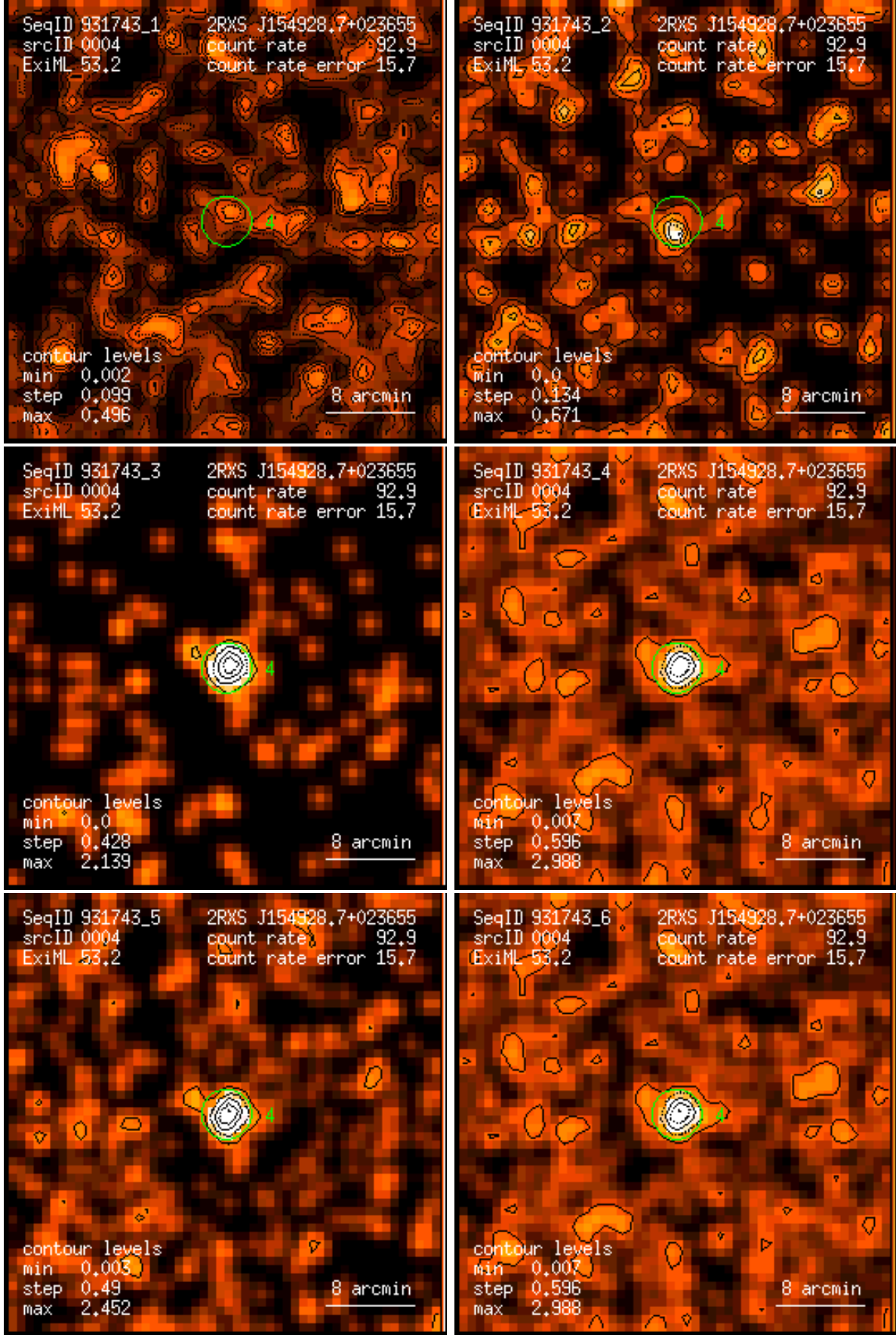
Figure 4: RASS 931743: detection 0004: band rate images, Gaussian filter: (1) PSPC channels 11 – 41, (2) 52 – 90, (3) 91 – 201, (4) 11 – 235, (5) 52 – 201, (6) 11 – 201. Broad band rates in counts/ks. Band rate contour levels in counts/ks/arcmin 2 .
