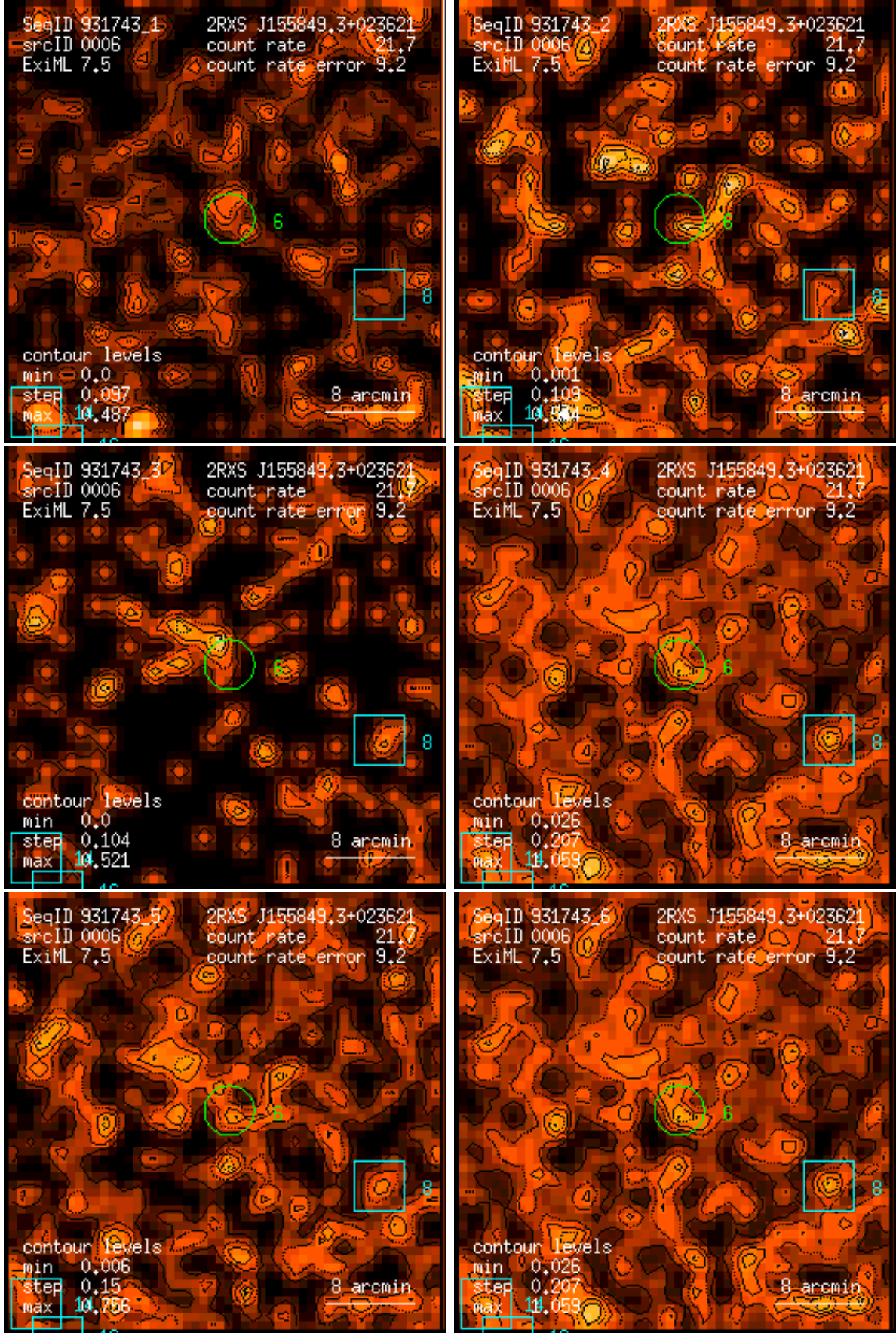
Figure 6: RASS 931743: detection 0006: band rate images, Gaussian filter: (1) PSPC channels 11 – 41, (2) 52 – 90, (3) 91 – 201, (4) 11 – 235, (5) 52 – 201, (6) 11 – 201. Broad band rates in counts/ks. Band rate contour levels in counts/ks/arcmin 2 .
