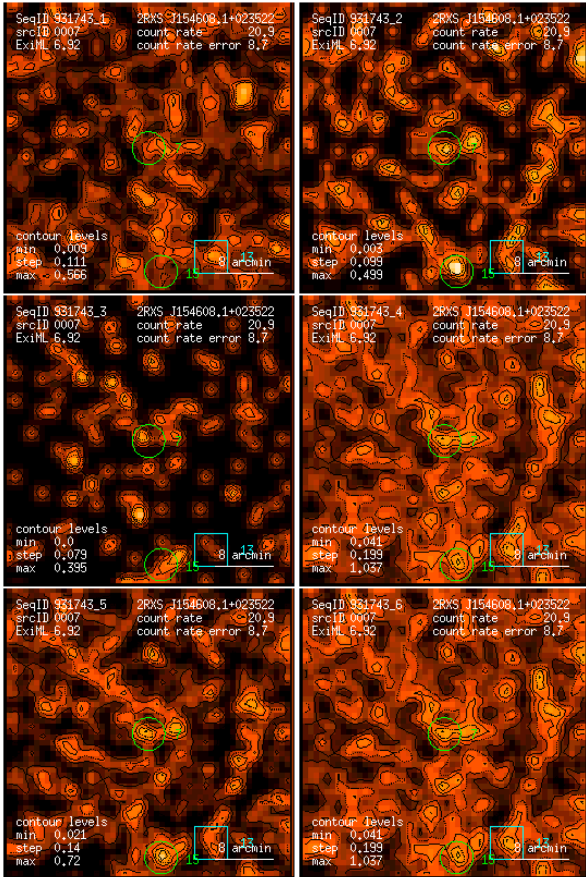
Figure 7: RASS 931743: detection 0007: band rate images, Gaussian filter: (1) PSPC channels 11 – 41, (2) 52 – 90, (3) 91 – 201, (4) 11 – 235, (5) 52 – 201, (6) 11 – 201. Broad band rates in counts/ks. Band rate contour levels in counts/ks/arcmin 2 .
