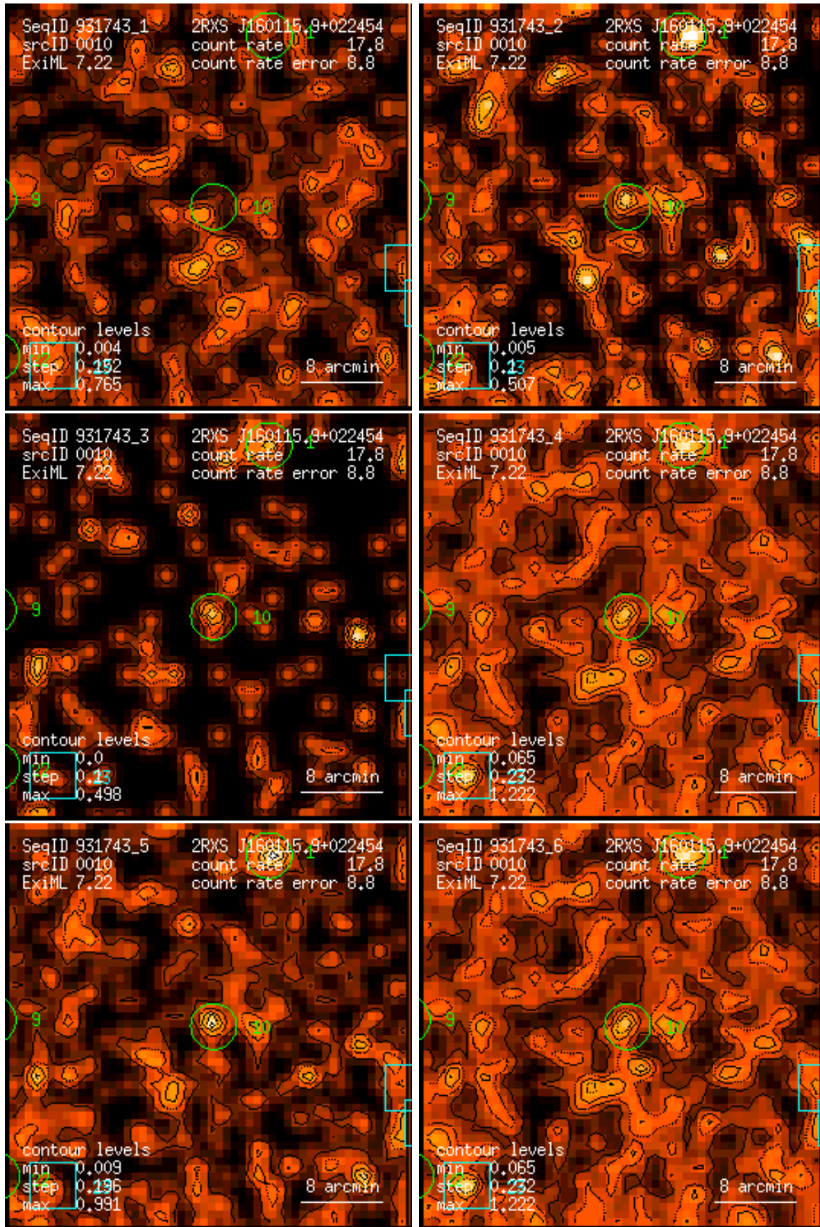
Figure 10: RASS 931743: detection 0010: band rate images, Gaussian filter: (1) PSPC channels 11 – 41, (2) 52 – 90, (3) 91 – 201, (4) 11 – 235, (5) 52 – 201, (6) 11 – 201. Broad band rates in counts/ks. Band rate contour levels in counts/ks/arcmin 2 .
