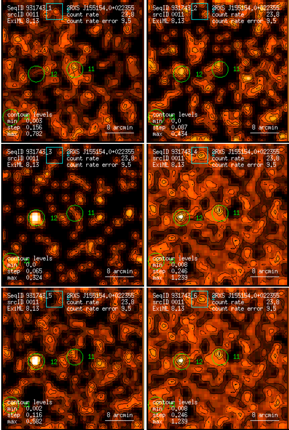
Figure 11: RASS 931743: detection 0011: band rate images, Gaussian filter: (1) PSPC channels 11 – 41, (2) 52 – 90, (3) 91 – 201, (4) 11 – 235, (5) 52 – 201, (6) 11 – 201. Broad band rates in counts/ks. Band rate contour levels in counts/ks/arcmin 2 .
