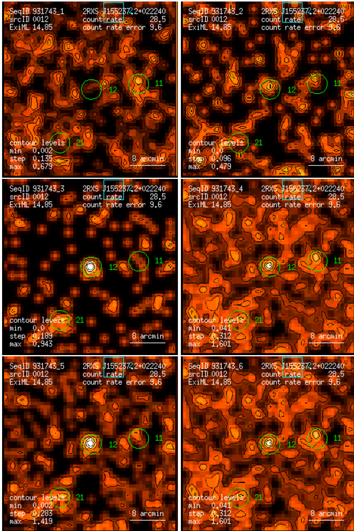
Figure 12: RASS 931743: detection 0012: band rate images, Gaussian filter: (1) PSPC channels 11 – 41, (2) 52 – 90, (3) 91 – 201, (4) 11 – 235, (5) 52 – 201, (6) 11 – 201. Broad band rates in counts/ks. Band rate contour levels in counts/ks/arcmin 2 .
