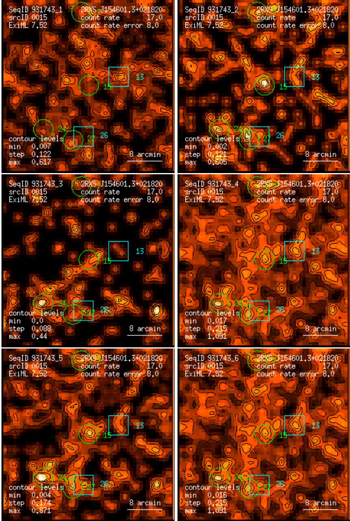
Figure 15: RASS 931743: detection 0015: band rate images, Gaussian filter: (1) PSPC channels 11 – 41, (2) 52 – 90, (3) 91 – 201, (4) 11 – 235, (5) 52 – 201, (6) 11 – 201. Broad band rates in counts/ks. Band rate contour levels in counts/ks/arcmin 2 .
