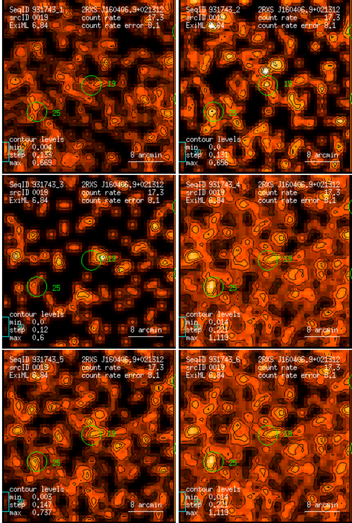
Figure 19: RASS 931743: detection 0019: band rate images, Gaussian filter: (1) PSPC channels 11 – 41, (2) 52 – 90, (3) 91 – 201, (4) 11 – 235, (5) 52 – 201, (6) 11 – 201. Broad band rates in counts/ks. Band rate contour levels in counts/ks/arcmin 2 .
