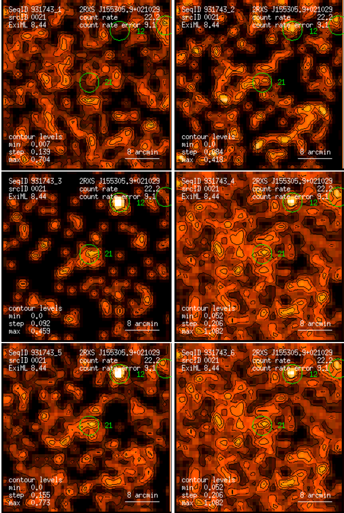
Figure 21: RASS 931743: detection 0021: band rate images, Gaussian filter: (1) PSPC channels 11 – 41, (2) 52 – 90, (3) 91 – 201, (4) 11 – 235, (5) 52 – 201, (6) 11 – 201. Broad band rates in counts/ks. Band rate contour levels in counts/ks/arcmin 2 .
